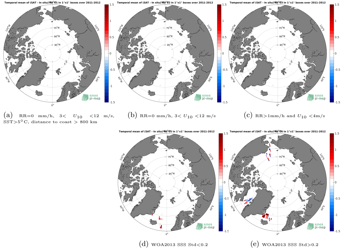
Figure 12: Temporal mean gridded over spatial boxes of size 1^{\circ}\times 1^{\circ} of \Delta\text{SSS} (Aquarius-L2-JPL-V5 - TSG-SAMOS) for 5 different subdatasets corresponding to: RR=0 mm/h, 3 < U_{10} < 12 m/s, SST > 5^{\circ}\text{C} , distance to coast > 800 km (a), RR=0 mm/h, 3 < U_{10} < 12 m/s (b), RR > 1 mm/h and U_{10} < 4 m/s (c), WOA2013 SSS Std < 0.2 (d), WOA2013 SSS Std > 0.2 (e).
