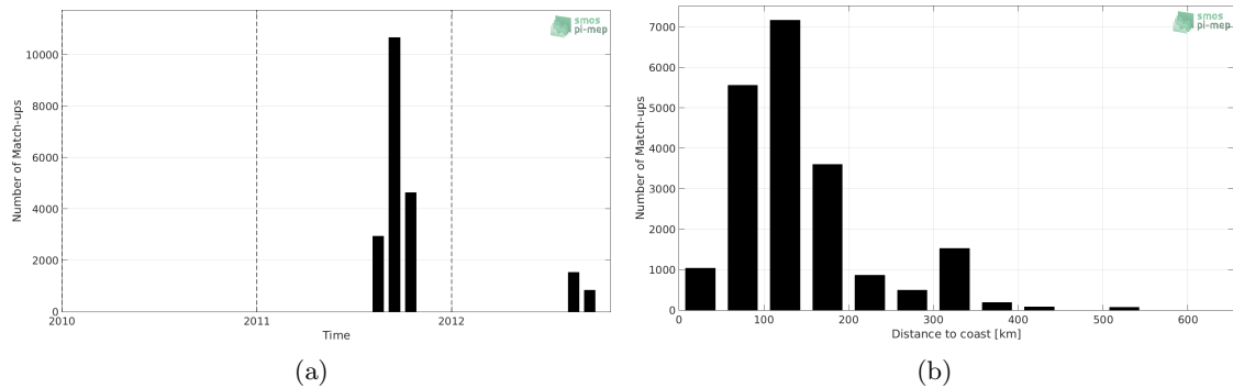
Figure 1: Number of match-ups between TSG-SAMOS and Aquarius-L2-JPL-V5 SSS as a function of time (a) and as function of the distance to coast (b) over the Arctic Ocean Pi-MEP region and for the full satellite product period.
