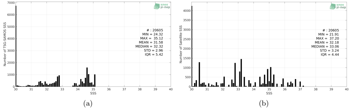
Figure 2: Histograms of SSS from TSG-SAMOS (a) and Aquarius-L2-JPL-V5 (b) considering all match-up pairs per bins of 0.1 over the Arctic Ocean Pi-MEP region and for the full satellite product period.
