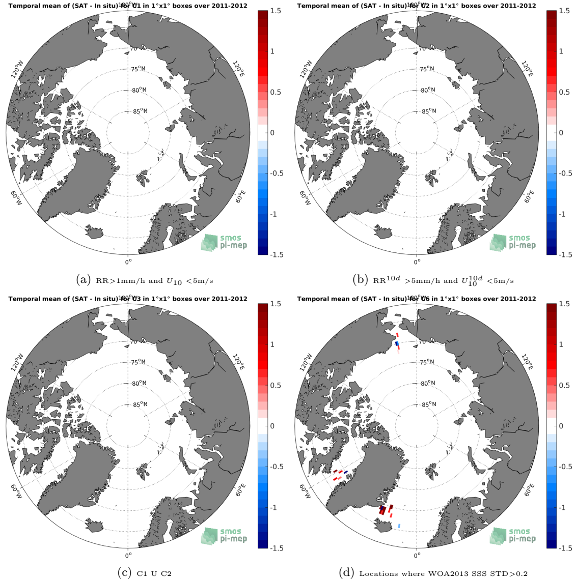
Figure 12: Temporal mean gridded over spatial boxes of size 1^\circ \times 1^\circ of \Delta SSS (Aquarius-L2-JPL-V5 - TSG-SAMOS) for 4 different subdatasets corresponding to: RR > 1\text{mm/h} and U_{10} < 5\text{m/s} (a), RR^{10d} > 5\text{mm/h} and U_{10}^{10d} < 5\text{m/s} (b), C1 U C2 (c), Locations where WOA2013 SSS STD > 0.2 (d).
