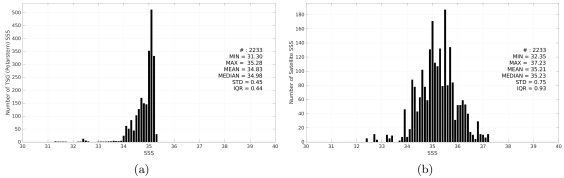
Figure 3: Histograms of SSS from TSG (Polarstern) (a) and Aquarius SSS L2 CAP v5 (JPL) (b) considering all match-up pairs per bins of 0.1 over the Arctic Ocean Pi-MEP region and for the full satellite product period.
