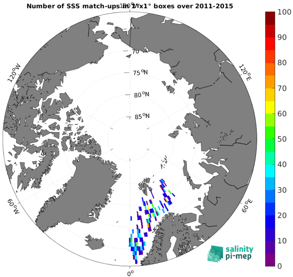
Figure 5: Number of SSS match-ups between TSG (Polarstern) SSS and the Aquarius SSS L2 CAP v5 (JPL) SSS product for the Arctic Ocean Pi-MEP region over 1^\circ \times 1^\circ boxes and for the full satellite product period.
