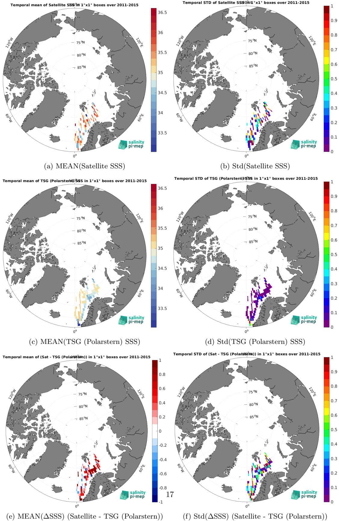
Figure 7: Temporal mean (left) and Std (right) of SSS from Aquarius SSS L2 CAP v5 (JPL) (top), TSG (Polarstern) (middle), and of \Delta SSS (Satellite - TSG (Polarstern)). Only match-up pairs are used to generate these maps.
