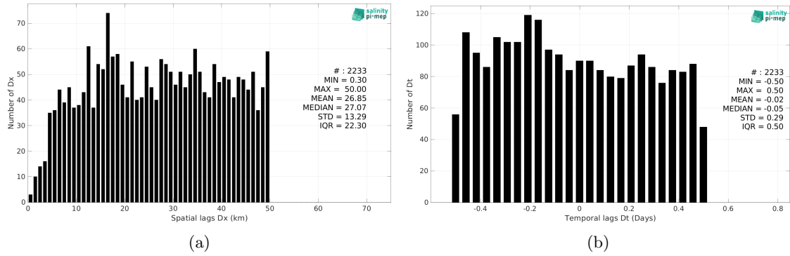
Figure 6: Histograms of the spatial (a) and temporal (b) lags between the location/time of the TSG (Polarstern) measurement and the date of the corresponding Aquarius SSS L2 CAP v5 (JPL) SSS pixel.
