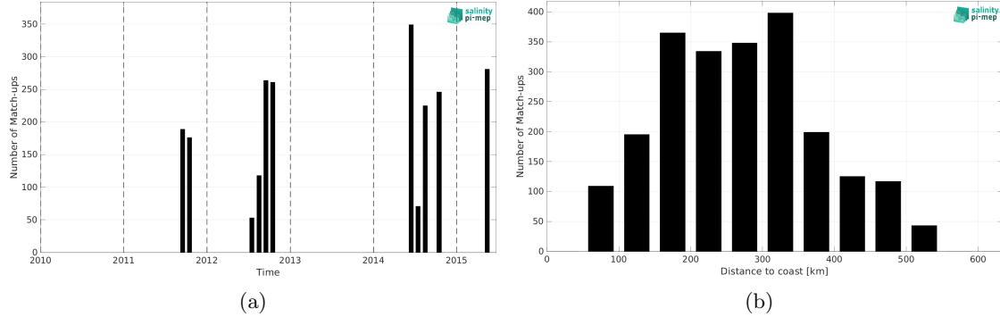
Figure 2: Number of match-ups between TSG (Polarstern) and Aquarius SSS L2 CAP v5 (JPL) SSS as a function of time (a) and as function of the distance to coast (b) over the Arctic Ocean Pi-MEP region and for the full satellite product period.
