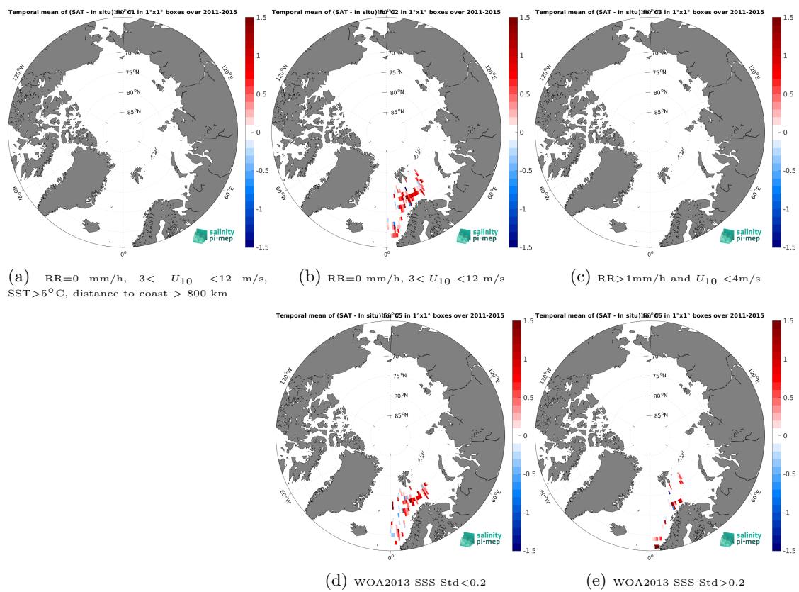
Figure 14: Temporal mean gridded over spatial boxes of size 1^\circ \times 1^\circ of \Delta SSS (Aquarius SSS L2 CAP v5 (JPL) - TSG (Polarstern)) for 5 different subdatasets corresponding to:RR=0 mm/h, 3 < U_{10} < 12 m/s, SST >5^\circ C, distance to coast > 800 km (a), RR=0 mm/h, 3 < U_{10} < 12 m/s (b), RR >1 mm/h and U_{10} < 4 m/s (c), WOA2013 SSS Std <0.2 (d), WOA2013 SSS Std >0.2 (e).
