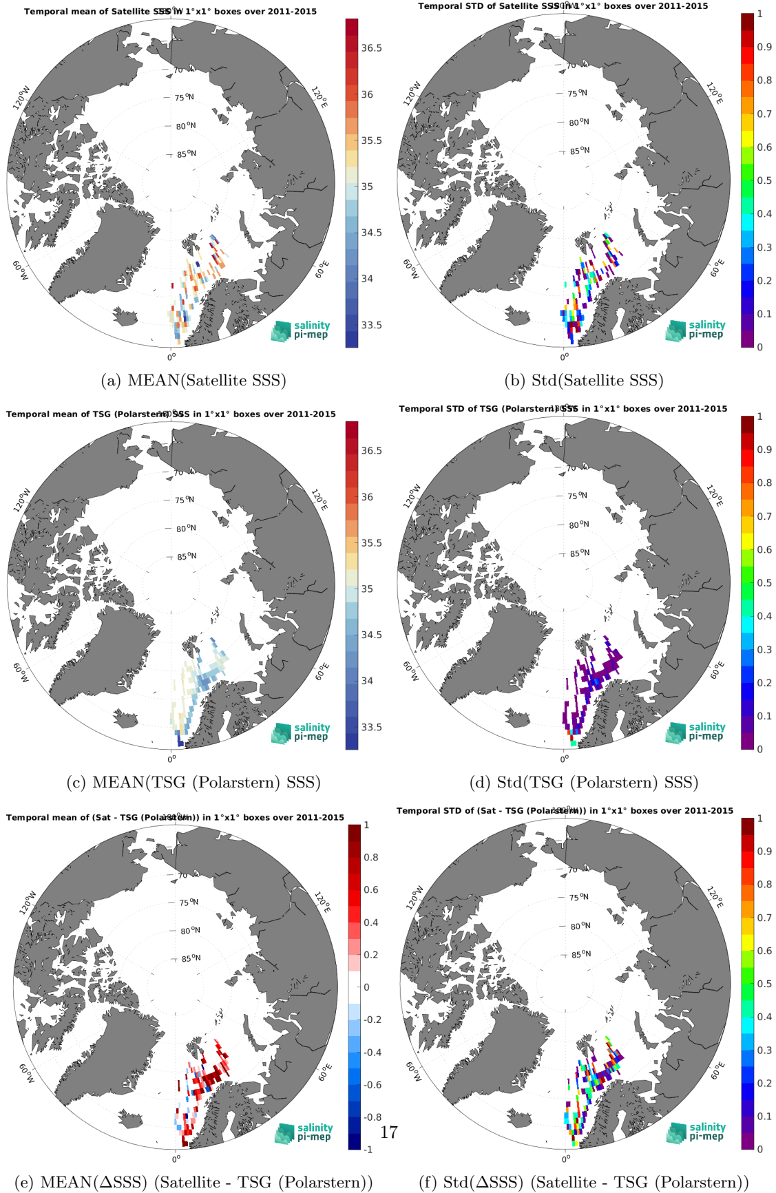
Figure 6: Temporal mean (left) and Std (right) of SSS from Aquarius SSS L2 CAP v5 (JPL) (top), TSG (Polarstern) (middle), and of \Delta SSS (Satellite - TSG (Polarstern)). Only match-up pairs are used to generate these maps.
