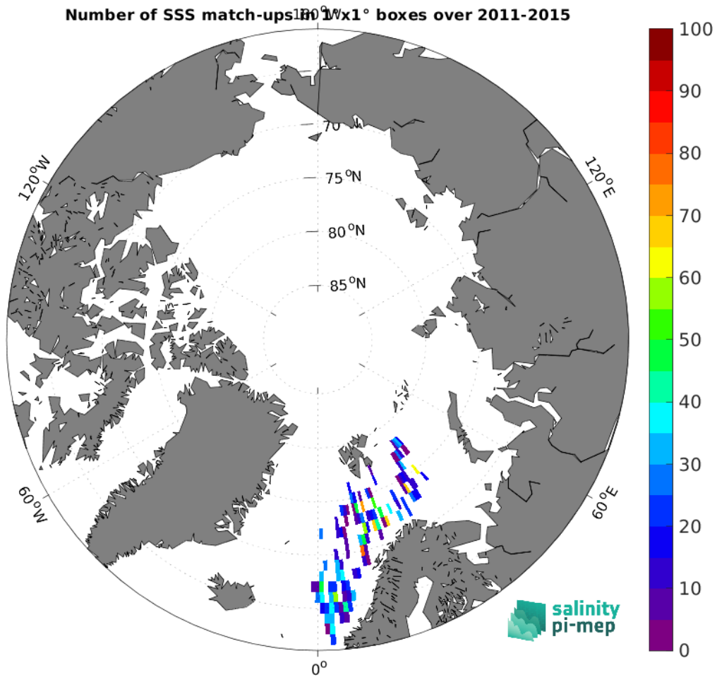
Figure 4: Number of SSS match-ups between TSG (Polarstern) SSS and the Aquarius SSS L2 CAP v5 (JPL) SSS product for the Arctic Ocean Pi-MEP region over 1^\circ \times 1^\circ boxes and for the full satellite product period.
