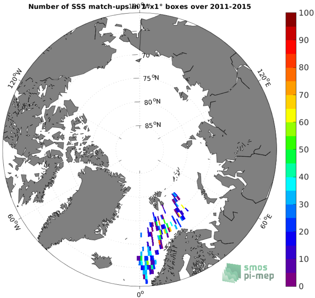
Figure 4: Number of SSS match-ups between TSG (Polarstern) SSS and the Aquarius SSS L2 CAP v5 (JPL) SSS product for the Arctic Ocean Pi-MEP region over 1^{\circ} \times 1^{\circ} boxes and for the full satellite product period.
