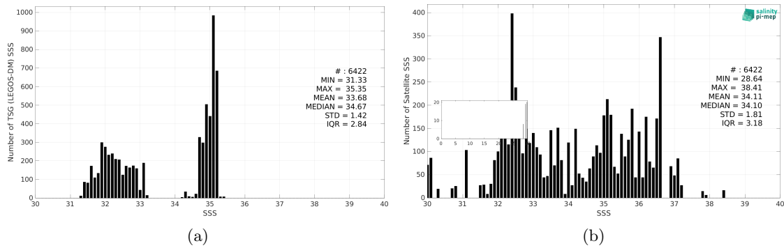
Figure 3: Histograms of SSS from TSG (LEGOS-DM) (a) and Aquarius SSS L2 CAP v5 (JPL) (b) considering all match-up pairs per bins of 0.1 over the Arctic Ocean Pi-MEP region and for the full satellite product period.
