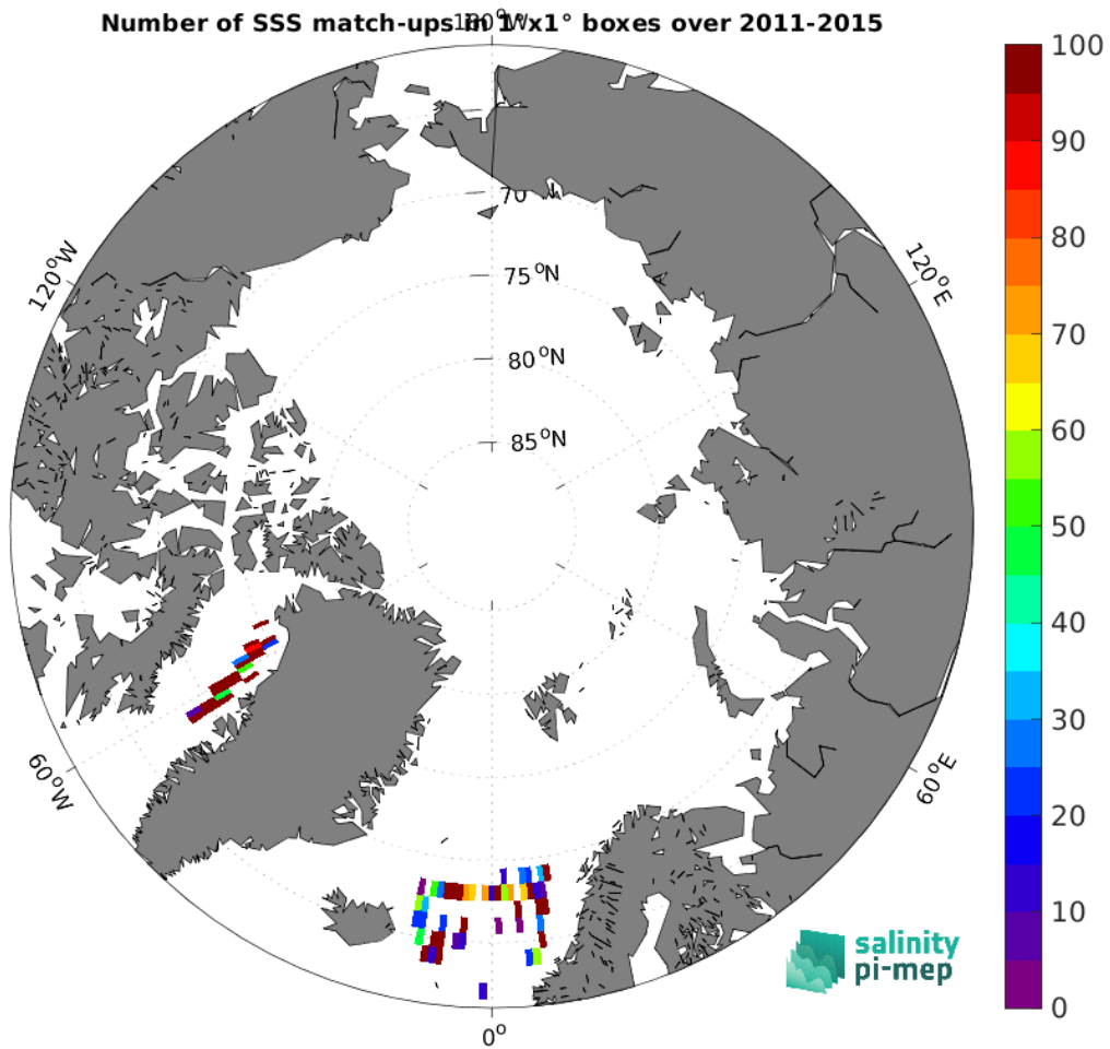
Figure 5: Number of SSS match-ups between TSG (LEGOS-DM) SSS and the Aquarius SSS L2 CAP v5 (JPL) SSS product for the Arctic Ocean Pi-MEP region over 1^\circ \times 1^\circ boxes and for the full satellite product period.
