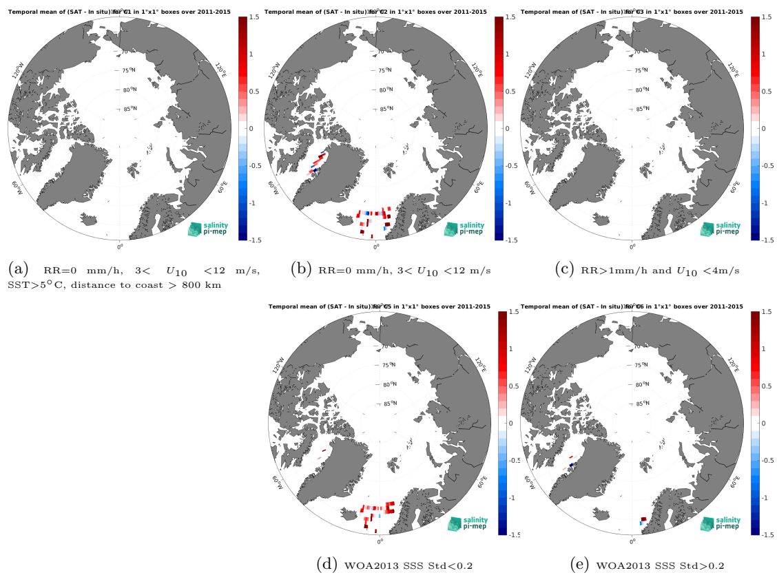
Figure 14: Temporal mean gridded over spatial boxes of size 1^\circ \times 1^\circ of \Delta SSS (Aquarius SSS L2 CAP v5 (JPL) - TSG (LEGOS-DM)) for 5 different subdatasets corresponding to: RR=0 mm/h, 3 < U_{10} < 12 m/s, SST > 5°C, distance to coast > 800 km (a), RR=0 mm/h, 3 < U_{10} < 12 m/s (b), RR > 1mm/h and U_{10} < 4 m/s (c), WOA2013 SSS Std < 0.2 (d), WOA2013 SSS Std > 0.2 (e).
