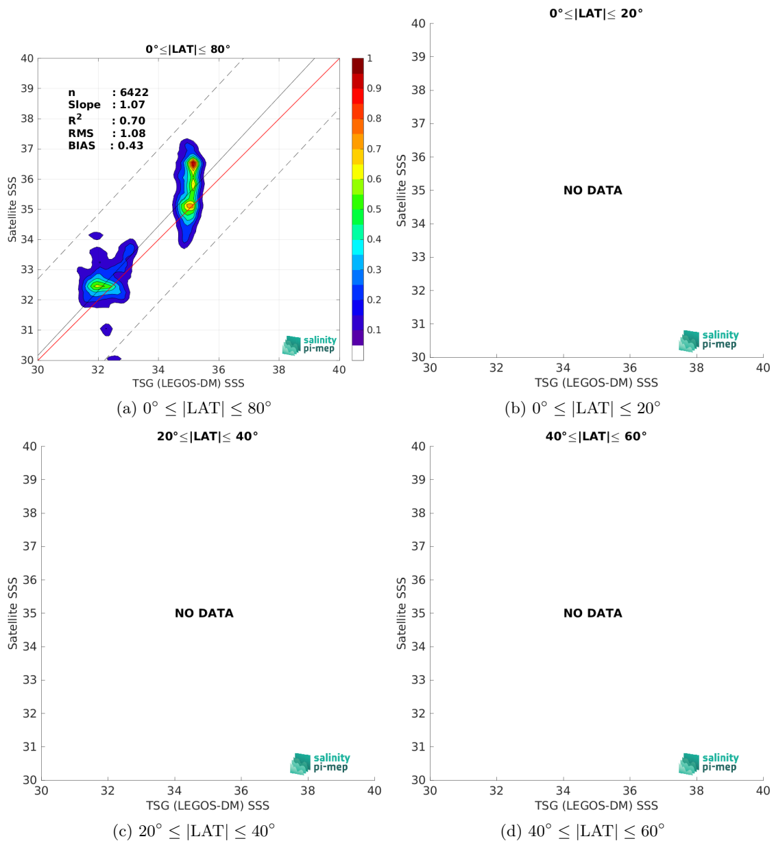
Figure 10: Contour maps of the concentration of Aquarius SSS L2 CAP v5 (JPL) SSS (y-axis) versus TSG (LEGOS-DM) SSS (x-axis) at match-up pairs for different latitude bands. For each plot, the red line shows x=y . The black thin and dashed lines indicate a linear fit through the data cloud and the \pm 95\% confidence levels, respectively. The number match-up pairs n , the slope and R^2 coefficient of the linear fit, the root mean square (RMS) and the mean bias between satellite and in situ data are indicated for each latitude band in each plots.
