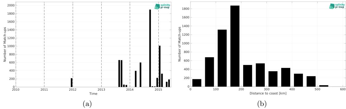
Figure 2: Number of match-ups between TSG (LEGOS-DM) and Aquarius SSS L2 CAP v5 (JPL) SSS as a function of time (a) and as function of the distance to coast (b) over the Arctic Ocean Pi-MEP region and for the full satellite product period.
