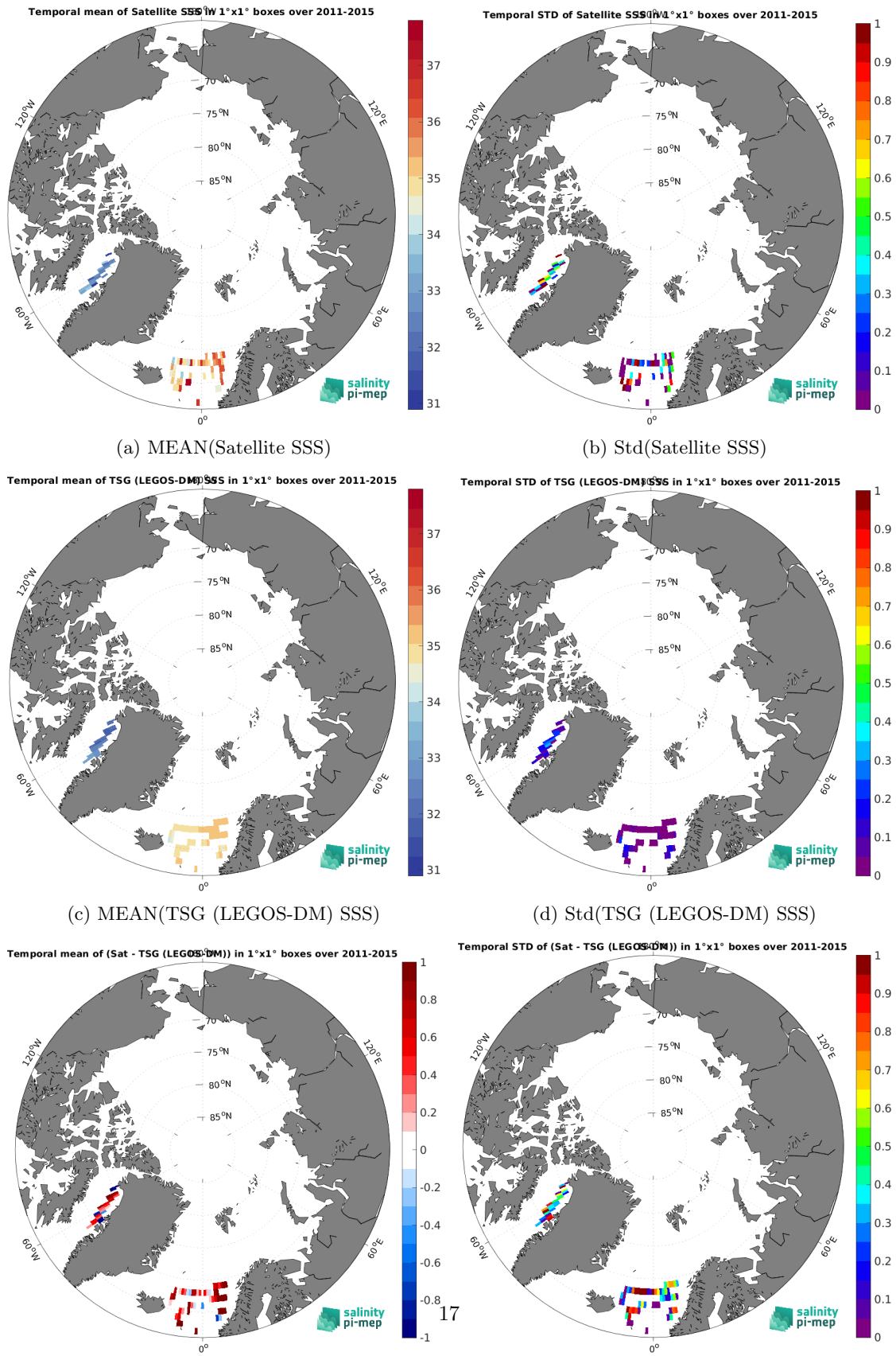
Figure 7: Temporal mean (left) and Std (right) of SSS from Aquarius SSS L2 CAP v5 (JPL) (top), TSG (LEGOS-DM) (middle), and of \Delta SSS (Satellite - TSG (LEGOS-DM)). Only match-up pairs are used to generate these maps.
