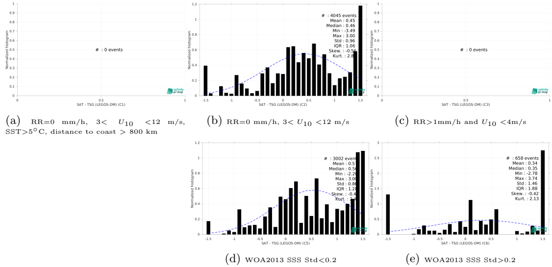
Figure 15: Normalized histogram of \Delta SSS (Aquarius SSS L2 CAP v5 (JPL) - TSG (LEGOS-DM)) for 5 different subdatasets corresponding to: RR=0 mm/h, 3 < U_{10} < 12 m/s, SST > 5°C, distance to coast > 800 km (a), RR=0 mm/h, 3 < U_{10} < 12 m/s (b), RR > 1mm/h and U_{10} < 4 m/s (c), WOA2013 SSS Std < 0.2 (d), WOA2013 SSS Std > 0.2 (e).
