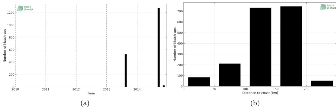
Figure 1: Number of match-ups between TSG-LEGOS-DM and Aquarius-L2-JPL-V5 SSS as a function of time (a) and as function of the distance to coast (b) over the Arctic Ocean Pi-MEP region and for the full satellite product period.
