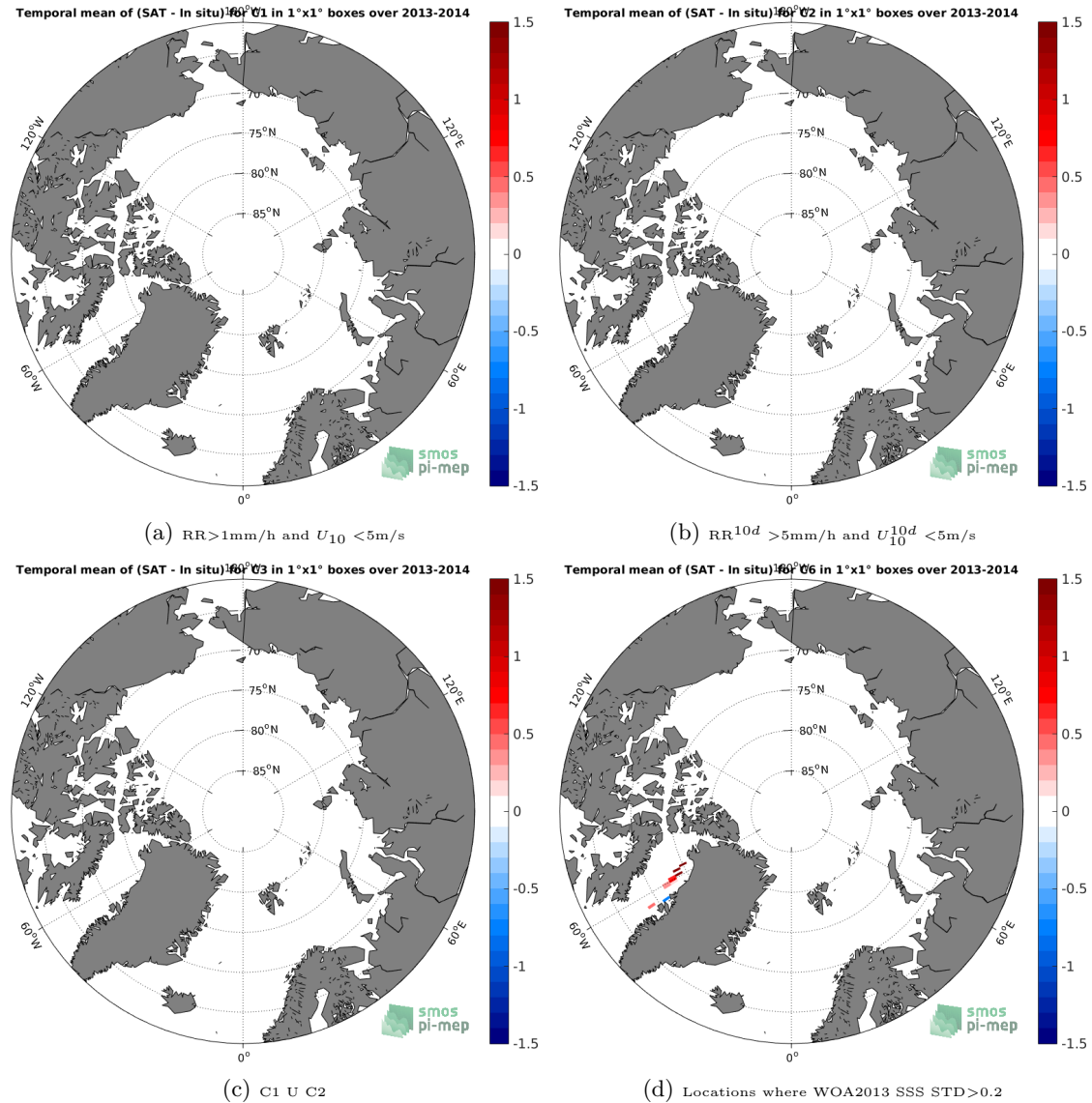
Figure 12: Temporal mean gridded over spatial boxes of size 1^\circ \times 1^\circ of \Delta SSS (Aquarius-L2-JPL-V5 - TSG-LEGOS-DM) for 4 different subdatasets corresponding to: RR > 1\text{mm/h} and U_{10} < 5\text{m/s} (a), RR^{10d} > 5\text{mm/h} and U_{10}^{10d} < 5\text{m/s} (b), C1 U C2 (c), Locations where WOA2013 SSS STD > 0.2 (d).
