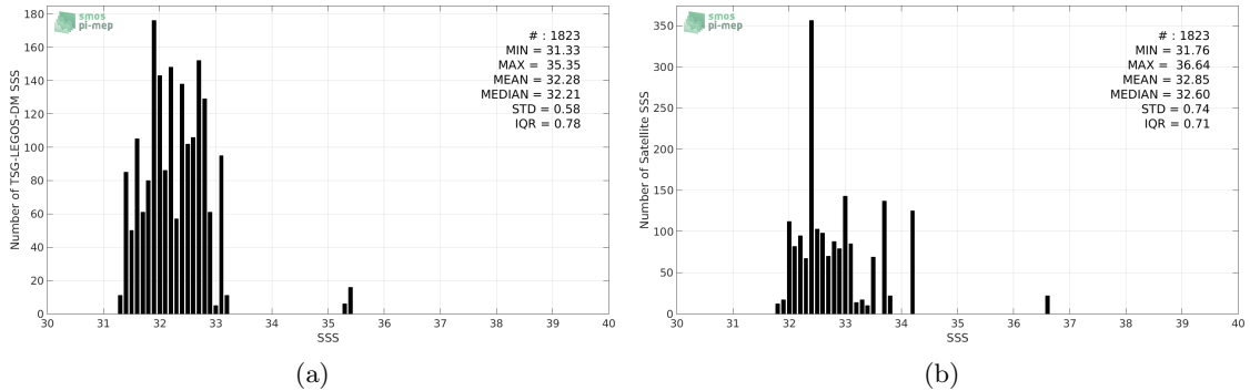
Figure 2: Histograms of SSS from TSG-LEGOS-DM (a) and Aquarius-L2-JPL-V5 (b) considering all match-up pairs per bins of 0.1 over the Arctic Ocean Pi-MEP region and for the full satellite product period.
