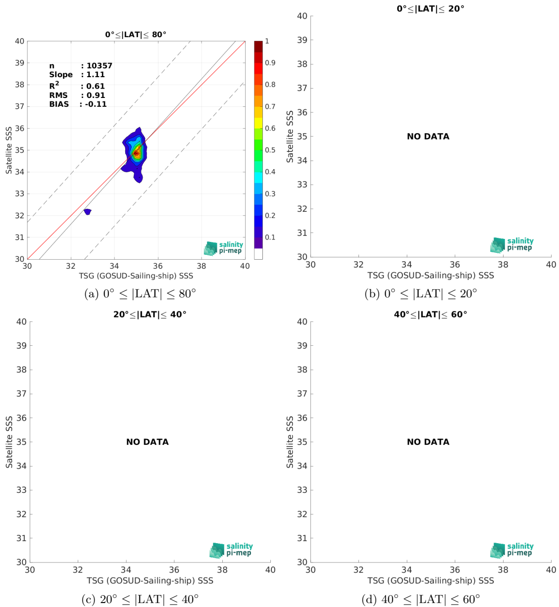
Figure 10: Contour maps of the concentration of Aquarius SSS L2 CAP v5 (JPL) SSS (y-axis) versus TSG (GOSUD-Sailing-ship) SSS (x-axis) at match-up pairs for different latitude bands. For each plot, the red line shows x=y . The black thin and dashed lines indicate a linear fit through the data cloud and the \pm 95\% confidence levels, respectively. The number match-up pairs n , the slope and R^2 coefficient of the linear fit, the root mean square (RMS) and the mean bias between satellite and in situ data are indicated for each latitude band in each plots.
