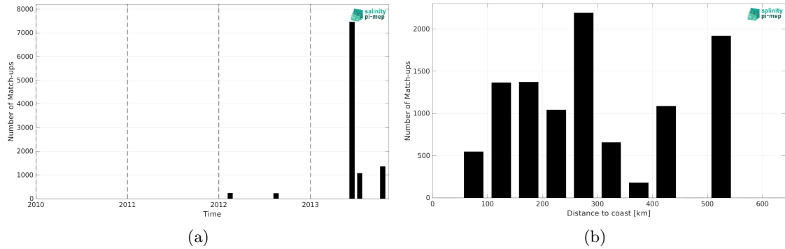
Figure 2: Number of match-ups between TSG (GOSUD-Sailing-ship) and Aquarius SSS L2 CAP v5 (JPL) SSS as a function of time (a) and as function of the distance to coast (b) over the Arctic Ocean Pi-MEP region and for the full satellite product period.
