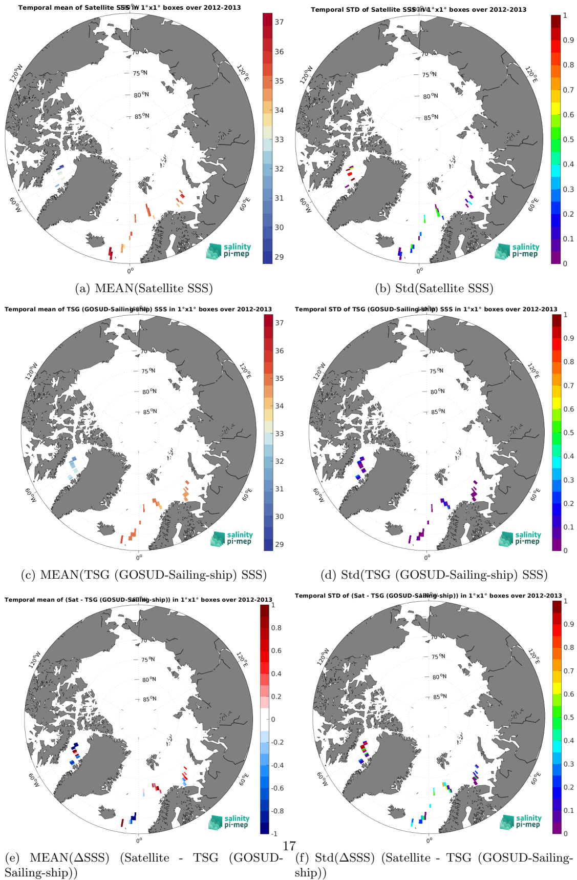
Figure 7: Temporal mean (left) and Std (right) of SSS from Aquarius SSS L2 CAP v5 (JPL) (top), TSG (GOSUD-Sailing-ship) (middle), and of \Delta SSS (Satellite - TSG (GOSUD-Sailing-ship)). Only match-up pairs are used to generate these maps.
