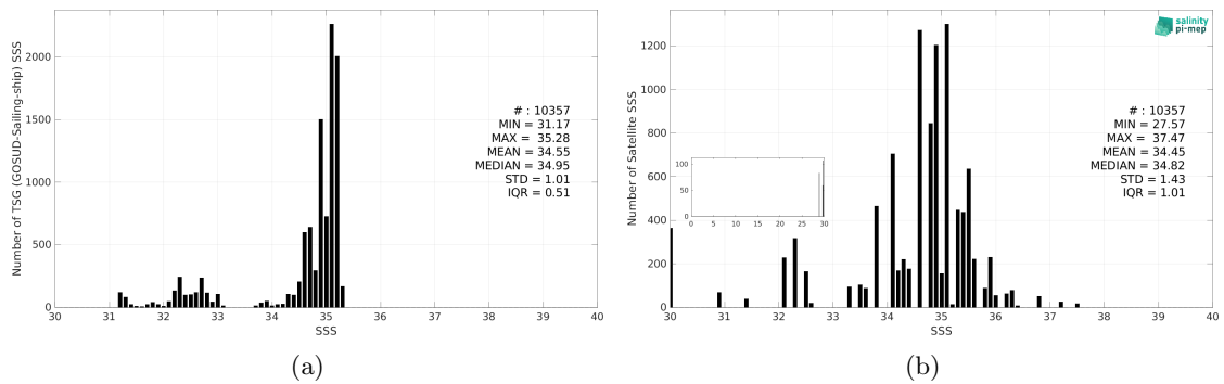
Figure 3: Histograms of SSS from TSG (GOSUD-Sailing-ship) (a) and Aquarius SSS L2 CAP v5 (JPL) (b) considering all match-up pairs per bins of 0.1 over the Arctic Ocean Pi-MEP region and for the full satellite product period.
