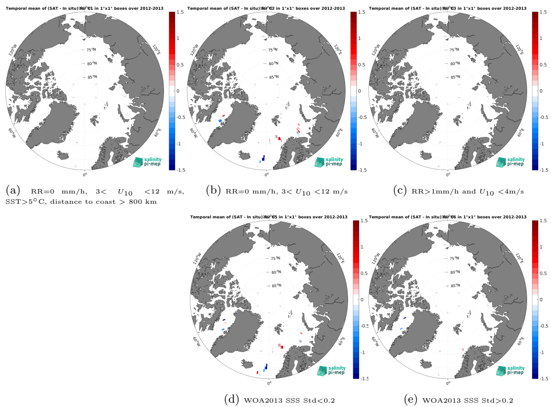
Figure 14: Temporal mean gridded over spatial boxes of size 1^\circ \times 1^\circ of \Delta\text{SSS} (Aquarius SSS L2 CAP v5 (JPL) - TSG (GOSUD-Sailing-ship)) for 5 different subdatasets corresponding to:RR=0 mm/h, 3 < U_{10} < 12 m/s, SST > 5°C, distance to coast > 800 km (a), RR=0 mm/h, 3 < U_{10} < 12 m/s (b), RR > 1mm/h and U_{10} < 4 m/s (c), WOA2013 SSS Std < 0.2 (d), WOA2013 SSS Std > 0.2 (e).
