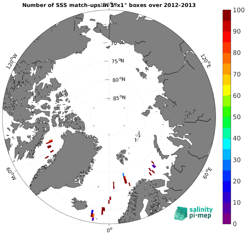
Figure 5: Number of SSS match-ups between TSG (GOSUD-Sailing-ship) SSS and the Aquarius SSS L2 CAP v5 (JPL) SSS product for the Arctic Ocean Pi-MEP region over 1^\circ \times 1^\circ boxes and for the full satellite product period.
