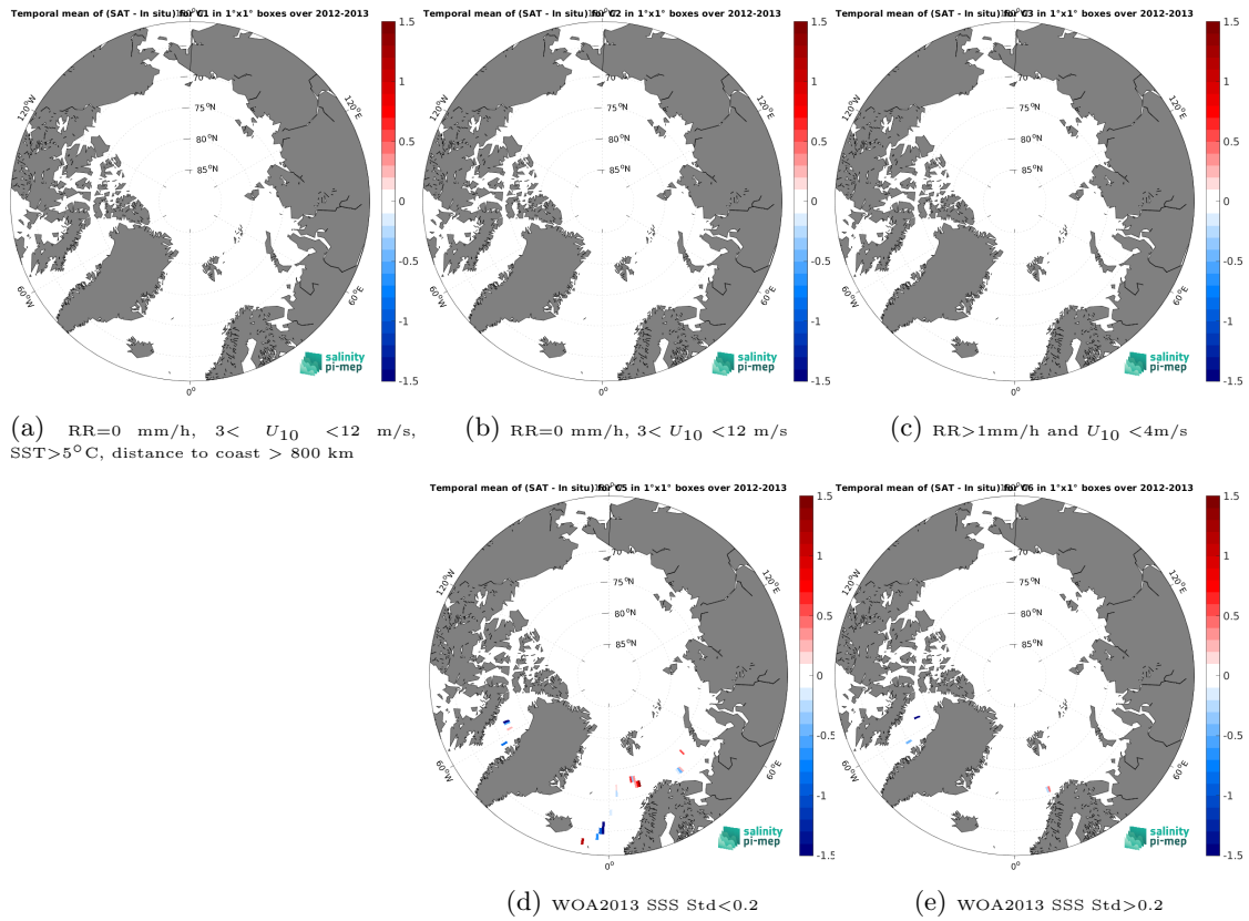
Figure 12: Temporal mean gridded over spatial boxes of size 1^{\circ} \times 1^{\circ} of \Delta SSS (Aquarius SSS L2 CAP v5 (JPL) - TSG (GOSUD-Sailing-ship)) for 5 different subdatasets corresponding to: RR=0 mm/h, 3 < U_{10} < 12 m/s, SST > 5^{\circ}C , distance to coast > 800 km (a), RR=0 mm/h, 3 < U_{10} < 12 m/s (b), RR > 1 mm/h and U_{10} < 4 m/s (c), WOA2013 SSS Std < 0.2 (d), WOA2013 SSS Std > 0.2 (e).
