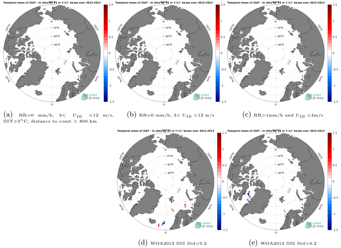
Figure 12: Temporal mean gridded over spatial boxes of size 1^\circ \times 1^\circ of \Delta\text{SSS} (Aquarius SSS L2 CAP v5 (JPL) - TSG (GOSUD-Sailing-ship)) for 5 different subdatasets corresponding to: RR=0 mm/h, 3 < U_{10} < 12 m/s, SST > 5^\circ\text{C} , distance to coast > 800 km (a), RR=0 mm/h, 3 < U_{10} < 12 m/s (b), RR > 1 mm/h and U_{10} < 4 m/s (c), WOA2013 SSS Std < 0.2 (d), WOA2013 SSS Std > 0.2 (e).
