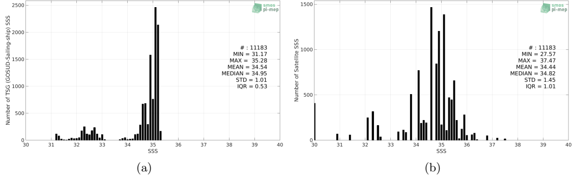
Figure 2: Histograms of SSS from TSG (GOSUD-Sailing-ship) (a) and Aquarius SSS L2 CAP v5 (JPL) (b) considering all match-up pairs per bins of 0.1 over the Arctic Ocean Pi-MEP region and for the full satellite product period.
