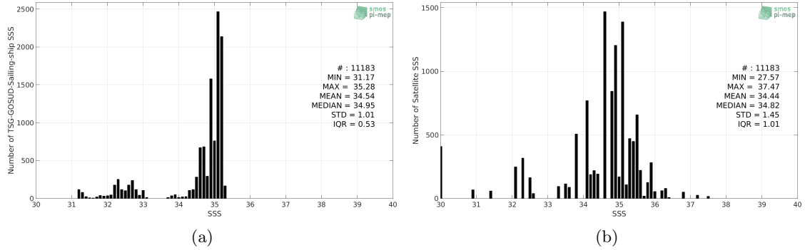
Figure 2: Histograms of SSS from TSG-GOSUD-Sailing-ship (a) and Aquarius-L2-JPL-V5 (b) considering all match-up pairs per bins of 0.1 over the Arctic Ocean Pi-MEP region and for the full satellite product period.
