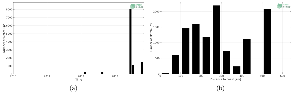
Figure 1: Number of match-ups between TSG-GOSUD-Sailing-ship and Aquarius-L2-JPL-V5 SSS as a function of time (a) and as function of the distance to coast (b) over the Arctic Ocean Pi-MEP region and for the full satellite product period.
