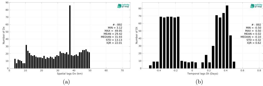
Figure 6: Histograms of the spatial (a) and temporal (b) lags between the location/time of the TSG (Amundsen) measurement and the date of the corresponding Aquarius SSS L2 CAP v5 (JPL) SSS pixel.
