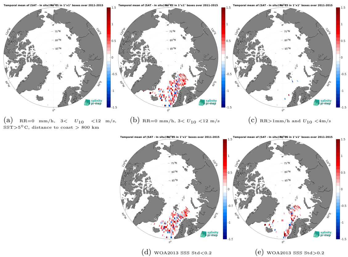
Figure 14: Temporal mean gridded over spatial boxes of size 1^\circ \times 1^\circ of \Delta SSS (Aquarius SSS L2 CAP v5 (JPL) - ICES) for 5 different subdatasets corresponding to:RR=0 mm/h, 3 < U_{10} < 12 m/s, SST>5°C, distance to coast > 800 km (a), RR=0 mm/h, 3 < U_{10} < 12 m/s (b), RR>1mm/h and U_{10} < 4 m/s (c), WOA2013 SSS Std<0.2 (d), WOA2013 SSS Std>0.2 (e).
