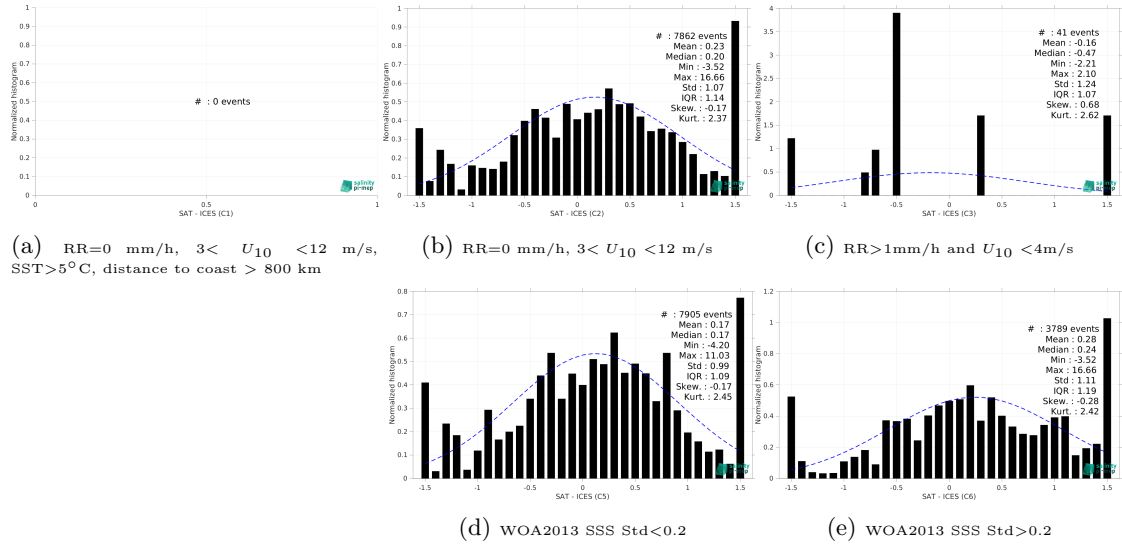
Figure 15: Normalized histogram of \Delta SSS (Aquarius SSS L2 CAP v5 (JPL) - ICES) for 5 different subdatasets corresponding to: RR=0 mm/h, 3 < U_{10} < 12 m/s, SST>5°C, distance to coast > 800 km (a), RR=0 mm/h, 3 < U_{10} < 12 m/s (b), RR>1mm/h and U_{10} < 4 m/s (c), WOA2013 SSS Std<0.2 (d), WOA2013 SSS Std>0.2 (e).
