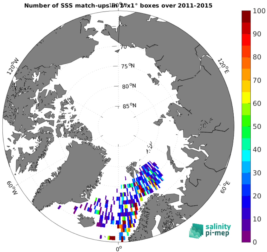
Figure 5: Number of SSS match-ups between ICES SSS and the Aquarius SSS L2 CAP v5 (JPL) SSS product for the Arctic Ocean Pi-MEP region over 1^\circ \times 1^\circ boxes and for the full satellite product period.
