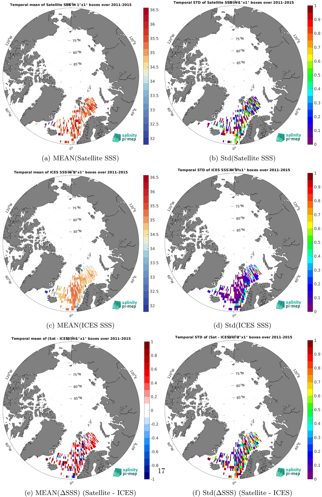
Figure 7: Temporal mean (left) and Std (right) of SSS from Aquarius SSS L2 CAP v5 (JPL) (top), ICES (middle), and of \Delta SSS (Satellite - ICES). Only match-up pairs are used to generate these maps.
