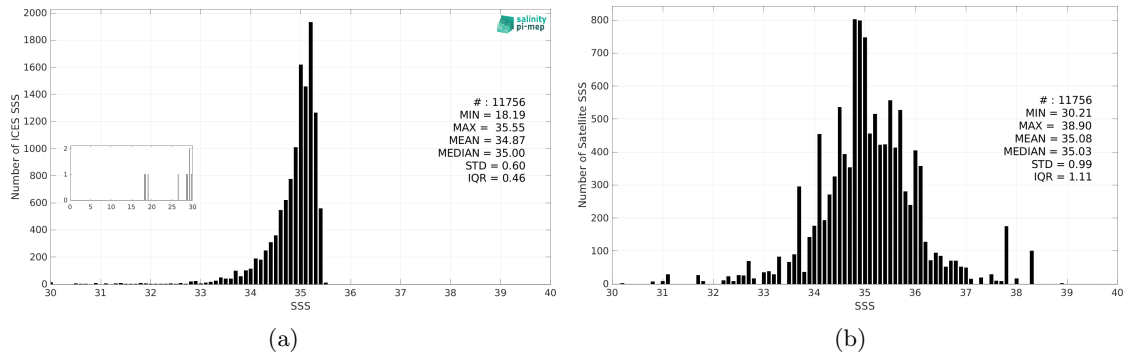
Figure 3: Histograms of SSS from ICES (a) and Aquarius SSS L2 CAP v5 (JPL) (b) considering all match-up pairs per bins of 0.1 over the Arctic Ocean Pi-MEP region and for the full satellite product period.
