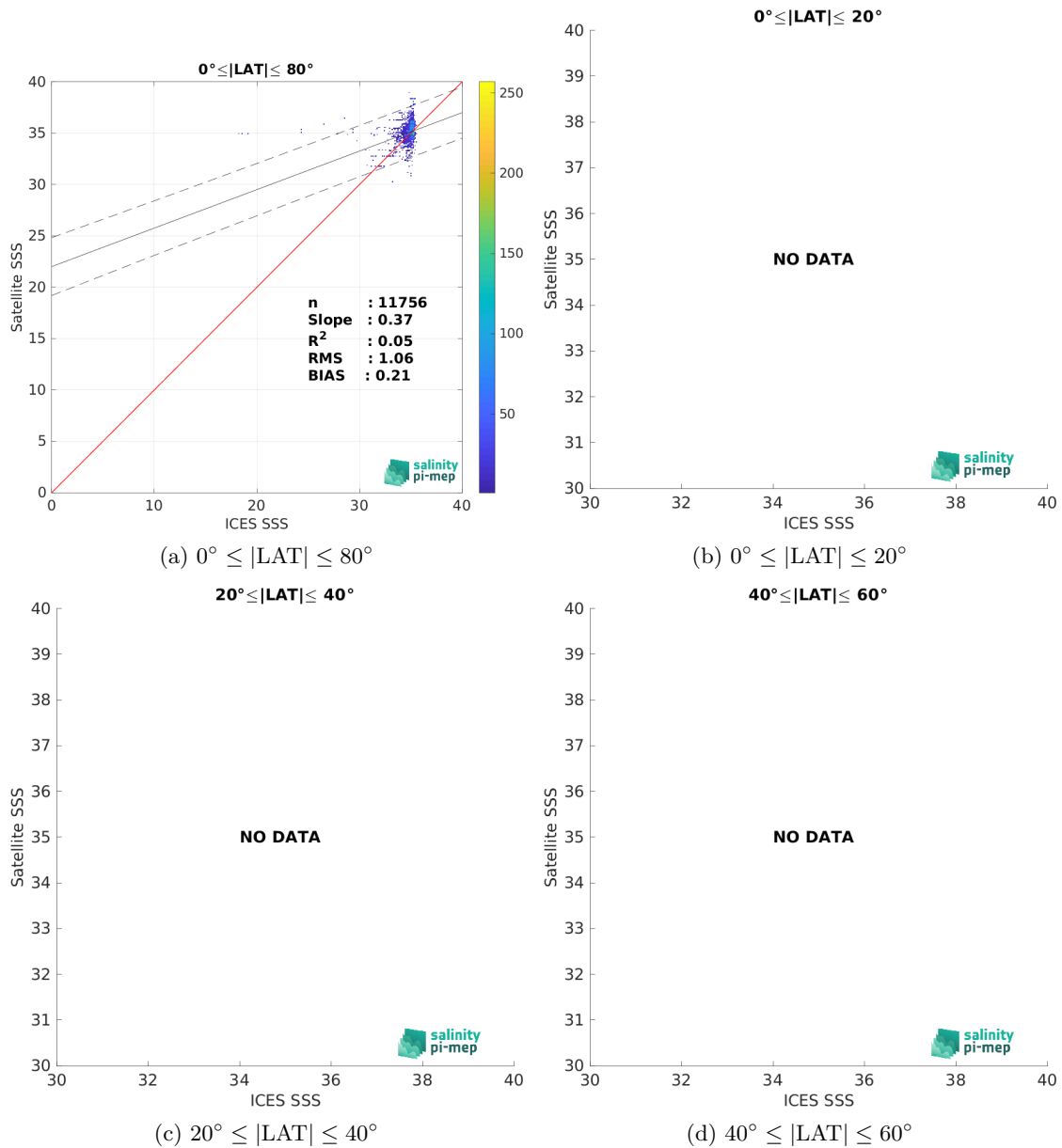
Figure 10: Contour maps of the concentration of Aquarius SSS L2 CAP v5 (JPL) SSS (y-axis) versus ICES SSS (x-axis) at match-up pairs for different latitude bands. For each plot, the red line shows x=y . The black thin and dashed lines indicate a linear fit through the data cloud and the \pm 95\% confidence levels, respectively. The number match-up pairs n , the slope and R^2 coefficient of the linear fit, the root mean square (RMS) and the mean bias between satellite and in situ data are indicated for each latitude band in each plots.
