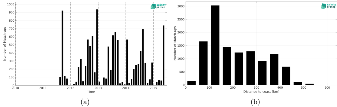
Figure 2: Number of match-ups between ICES and Aquarius SSS L2 CAP v5 (JPL) SSS as a function of time (a) and as function of the distance to coast (b) over the Arctic Ocean Pi-MEP region and for the full satellite product period.
