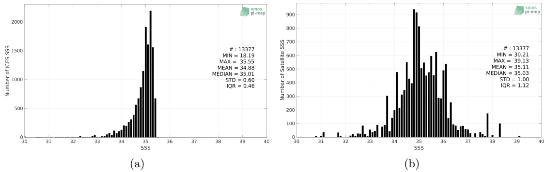
Figure 2: Histograms of SSS from ICES (a) and Aquarius SSS L2 CAP v5 (JPL) (b) considering all match-up pairs per bins of 0.1 over the Arctic Ocean Pi-MEP region and for the full satellite product period.
