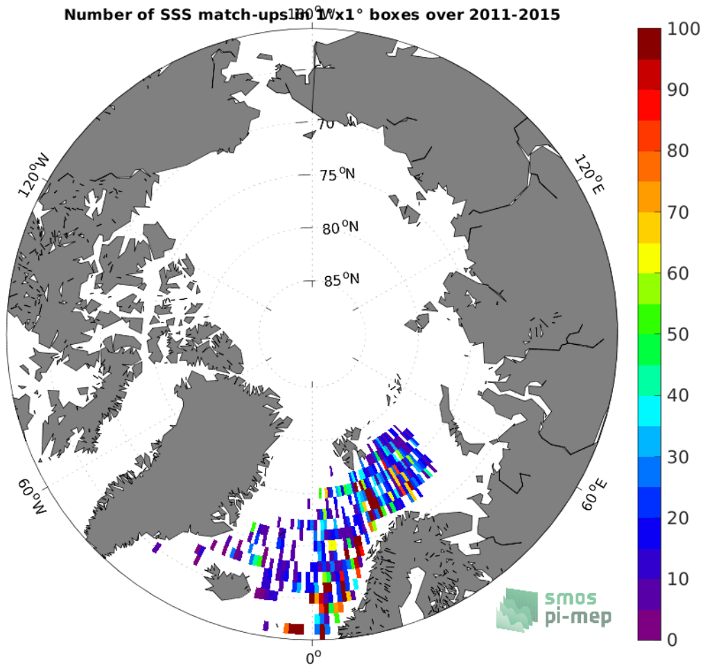
Figure 4: Number of SSS match-ups between ICES SSS and the Aquarius SSS L2 CAP v5 (JPL) SSS product for the Arctic Ocean Pi-MEP region over 1^\circ \times 1^\circ boxes and for the full satellite product period.
