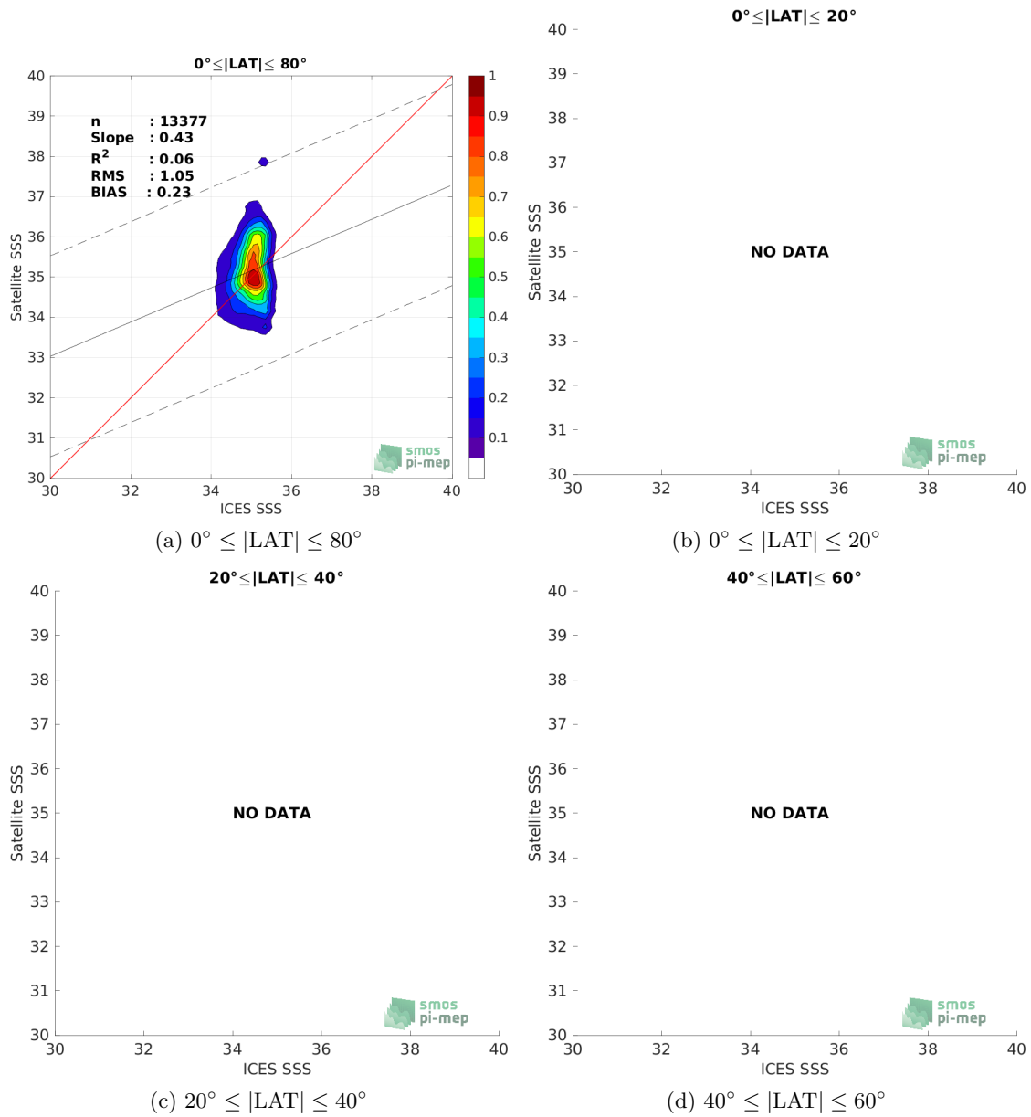
Figure 9: Contour maps of the concentration of Aquarius SSS L2 CAP v5 (JPL) SSS (y-axis) versus ICES SSS (x-axis) at match-up pairs for different latitude bands. For each plot, the red line shows x=y . The black thin and dashed lines indicate a linear fit through the data cloud and the \pm 95\% confidence levels, respectively. The number match-up pairs n , the slope and R^2 coefficient of the linear fit, the root mean square (RMS) and the mean bias between satellite and in situ data are indicated for each latitude band in each plots.
