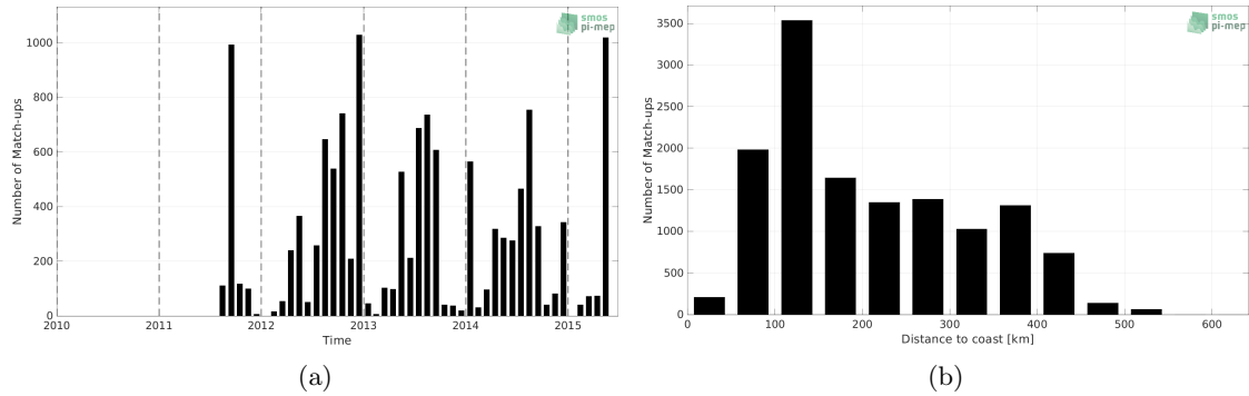
Figure 1: Number of match-ups between ICES and Aquarius SSS L2 CAP v5 (JPL) SSS as a function of time (a) and as function of the distance to coast (b) over the Arctic Ocean Pi-MEP region and for the full satellite product period.
