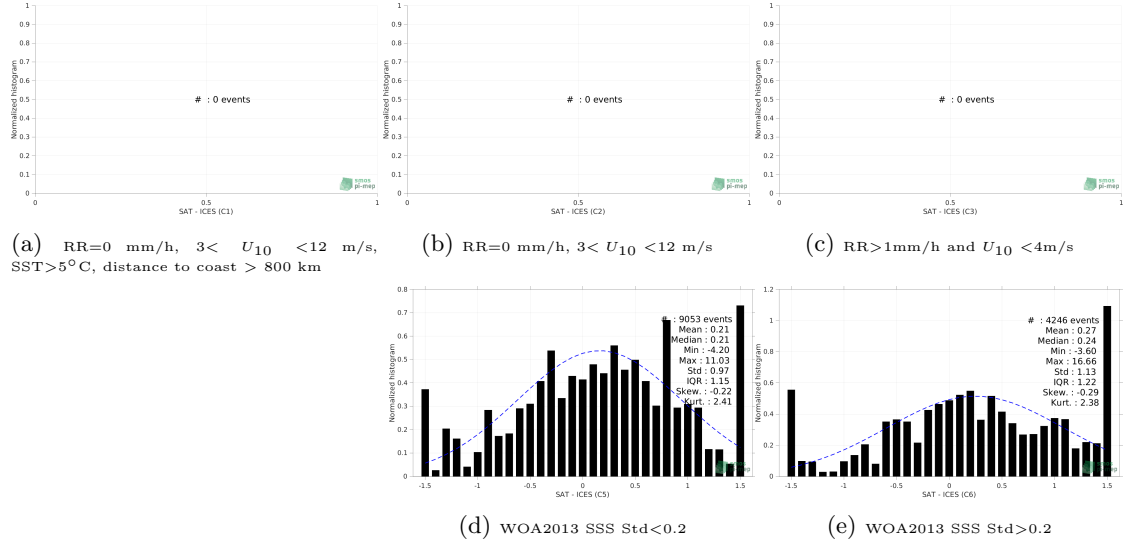
Figure 13: Normalized histogram of \Delta SSS (Aquarius SSS L2 CAP v5 (JPL) - ICES) for 5 different subdatasets corresponding to: RR=0 mm/h, 3 < U_{10} < 12 m/s, SST > 5°C, distance to coast > 800 km (a), RR=0 mm/h, 3 < U_{10} < 12 m/s (b), RR > 1mm/h and U_{10} < 4 m/s (c), WOA2013 SSS Std < 0.2 (d), WOA2013 SSS Std > 0.2 (e).
