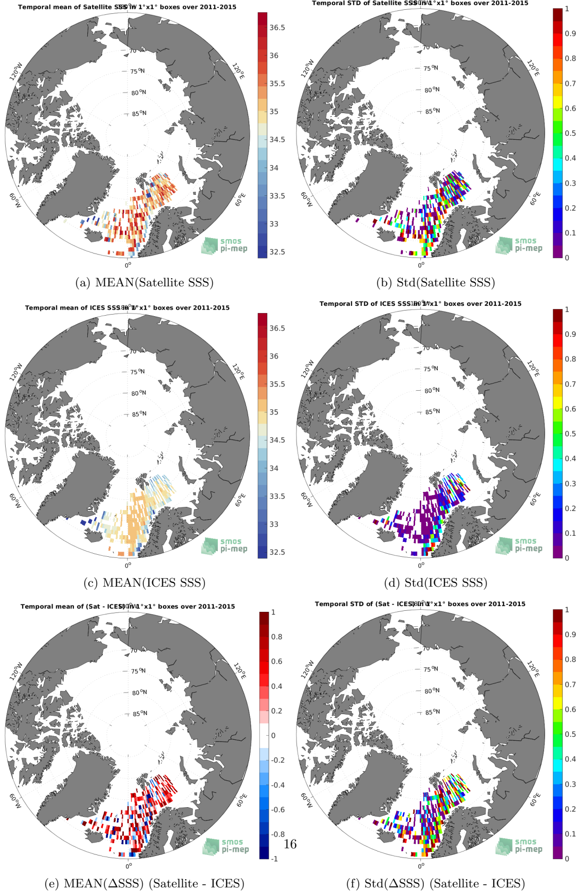
Figure 6: Temporal mean (left) and Std (right) of SSS from Aquarius SSS L2 CAP v5 (JPL) (top), ICES (middle), and of \Delta SSS (Satellite - ICES). Only match-up pairs are used to generate these maps.
