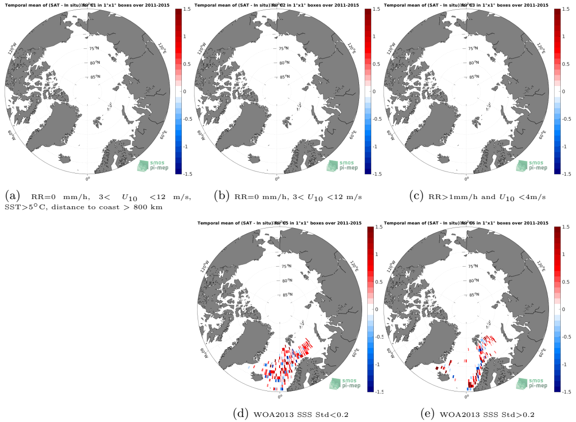
Figure 12: Temporal mean gridded over spatial boxes of size 1^{\circ}\times 1^{\circ} of \Delta\text{SSS} (Aquarius SSS L2 CAP v5 (JPL) - ICES) for 5 different subdatasets corresponding to:RR=0 mm/h, 3 < U_{10} < 12 m/s, SST > 5^{\circ}\text{C} , distance to coast > 800 km (a), RR=0 mm/h, 3 < U_{10} < 12 m/s (b), RR > 1 mm/h and U_{10} < 4 m/s (c), WOA2013 SSS Std < 0.2 (d), WOA2013 SSS Std > 0.2 (e).
