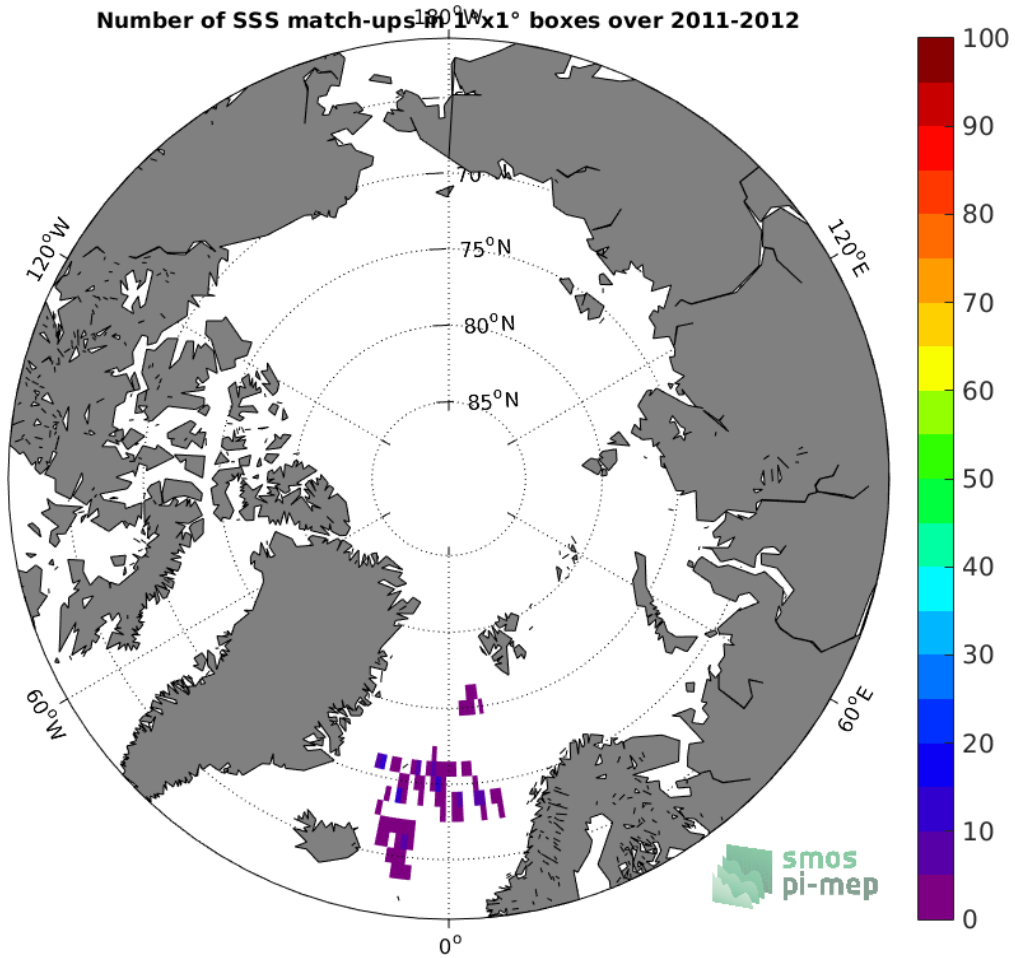
Figure 3: Number of SSS match-ups between Surface drifters SSS and the Aquarius-L2-JPL-V5 SSS product for the Arctic Ocean Pi-MEP region over 1^\circ \times 1^\circ boxes and for the full satellite product period.
