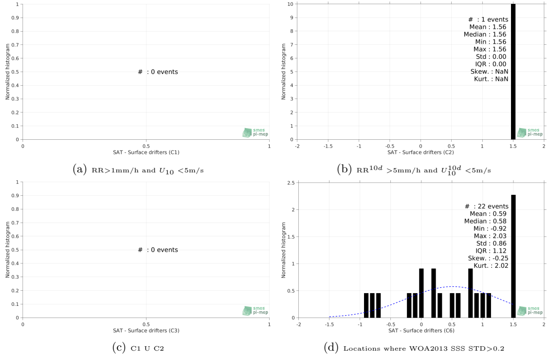
Figure 12: Normalized histogram of \Delta\text{SSS} (Aquarius-L2-JPL-V5 - Surface drifters) for 6 different subdatasets corresponding to: RR > 1\text{mm/h} and U_{10} < 5\text{m/s} (a), RR^{10d} > 5\text{mm/h} and U_{10}^{10d} < 5\text{m/s} (b), C1 \cup C2 (c), Locations where WOA2013 SSS STD > 0.2 (d).
