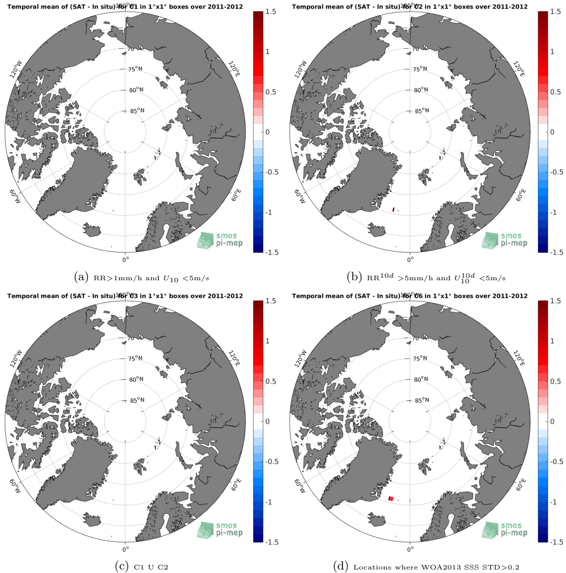
Figure 11: Temporal mean gridded over spatial boxes of size 1^\circ \times 1^\circ of \Delta SSS (Aquarius-L2-JPL-V5 - Surface drifters) for 4 different subdatasets corresponding to: RR > 1\text{mm/h} and U_{10} < 5\text{m/s} (a), RR^{10d} > 5\text{mm/h} and U_{10}^{10d} < 5\text{m/s} (b), C1 U C2 (c), Locations where WOA2013 SSS STD > 0.2 (d).
