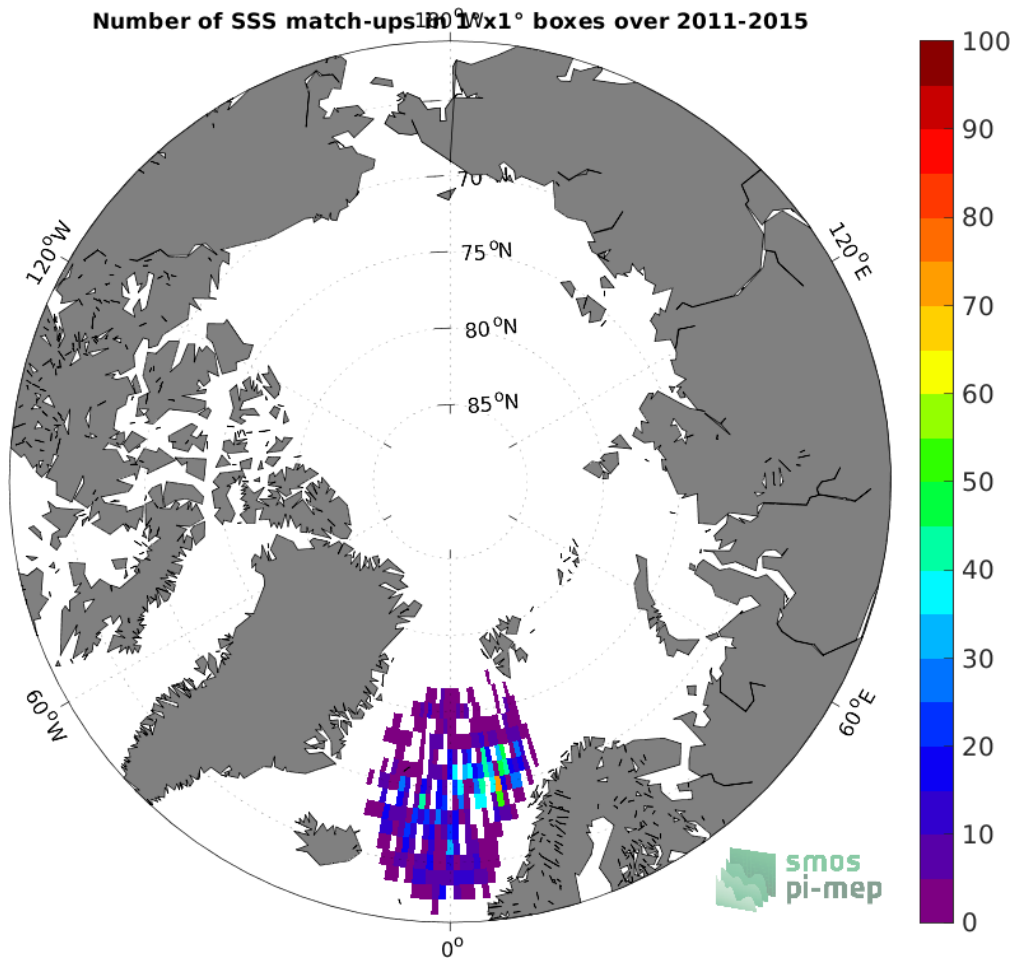
Figure 4: Number of SSS match-ups between Argo SSS and the Aquarius SSS L2 CAP v5 (JPL) SSS product for the Arctic Ocean Pi-MEP region over 1^{\circ} \times 1^{\circ} boxes and for the full satellite product period.
