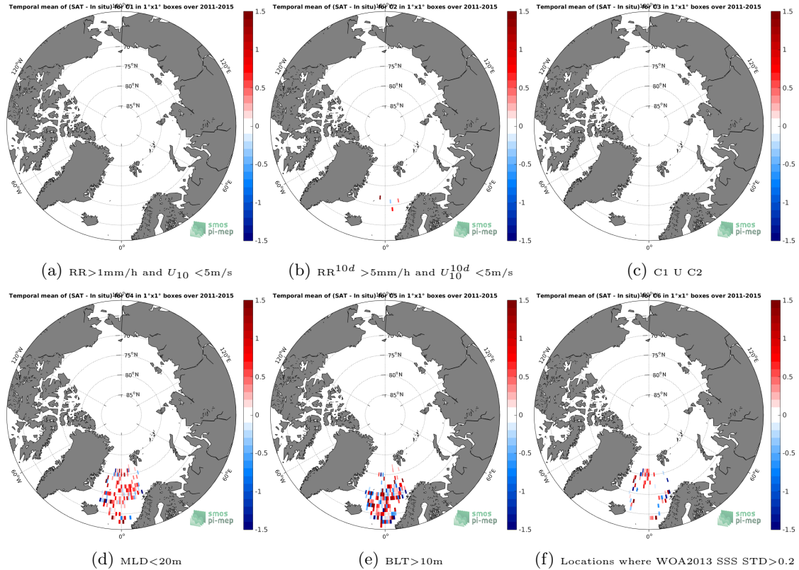
Figure 12: Temporal mean gridded over spatial boxes of size 1^\circ \times 1^\circ of \Delta SSS (Aquarius-L2-JPL-V5 - Argo) for 6 different subdatasets corresponding to: RR > 1\text{mm/h} and U_{10} < 5\text{m/s} (a), RR^{10d} > 5\text{mm/h} and U_{10}^{10d} < 5\text{m/s} (b), C1 U C2 (c), MLD < 20\text{m} (d), BLT > 10\text{m} (e), Locations where WOA2013 SSS STD > 0.2 (f).
