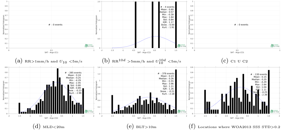
Figure 13: Normalized histogram of \Delta\text{SSS} (Aquarius-L2-JPL-V5 - Argo) for 6 different sub-datasets corresponding to: \text{RR} > 1\text{mm/h} and U_{10} < 5\text{m/s} (a), \text{RR}^{10d} > 5\text{mm/h} and U_{10}^{10d} < 5\text{m/s} (b), C1 U C2 (c), \text{MLD} < 20\text{m} (d), \text{BLT} > 10\text{m} (e), Locations where WOA2013 SSS \text{STD} > 0.2 (f).
