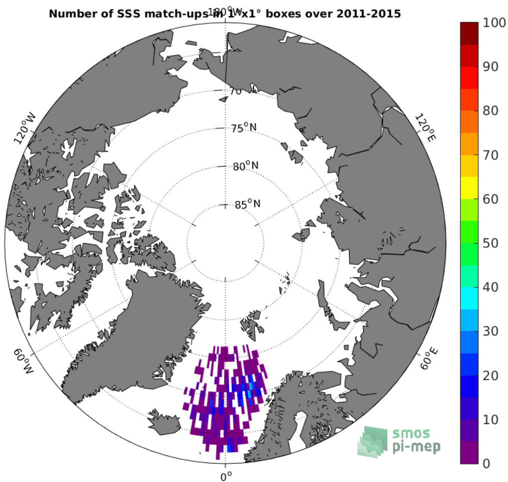
Figure 4: Number of SSS match-ups between Argo SSS and the Aquarius-L2-JPL-V5 SSS product for the Arctic Ocean Pi-MEP region over 1°x1° boxes and for the full satellite product period.
