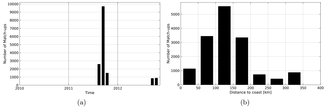
Figure 1: Number of match-ups between TSG-SAMOS and AQUARIUS-L2-JPL-V4 SSS as a function of time (a) and as function of the distance to coast (b) over the Arctic Ocean Pi-MEP region and for the full satellite product period.
