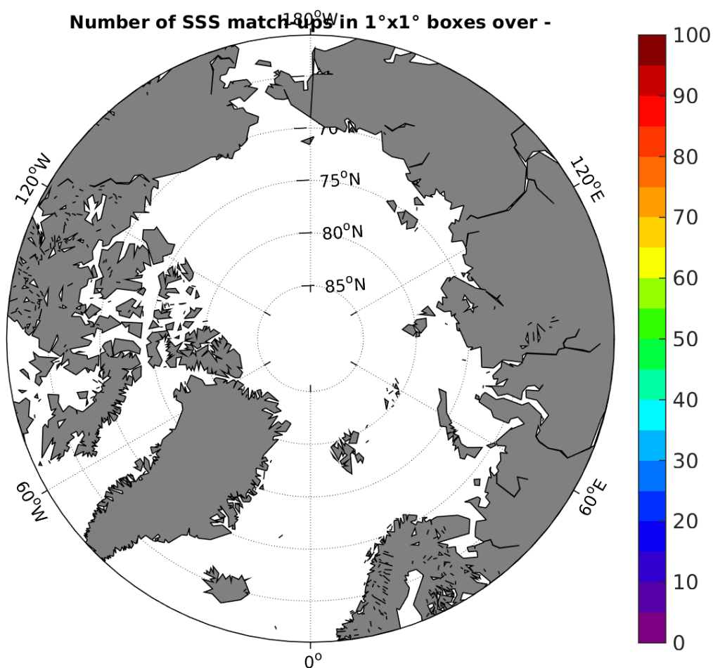
Figure 4: Number of SSS match-ups between TSG-GOSUD-Research-vessel SSS and the AQUARIUS-L2-JPL-V4 SSS product for the Arctic Ocean Pi-MEP region over 1°x1° boxes and for the full satellite product period.
