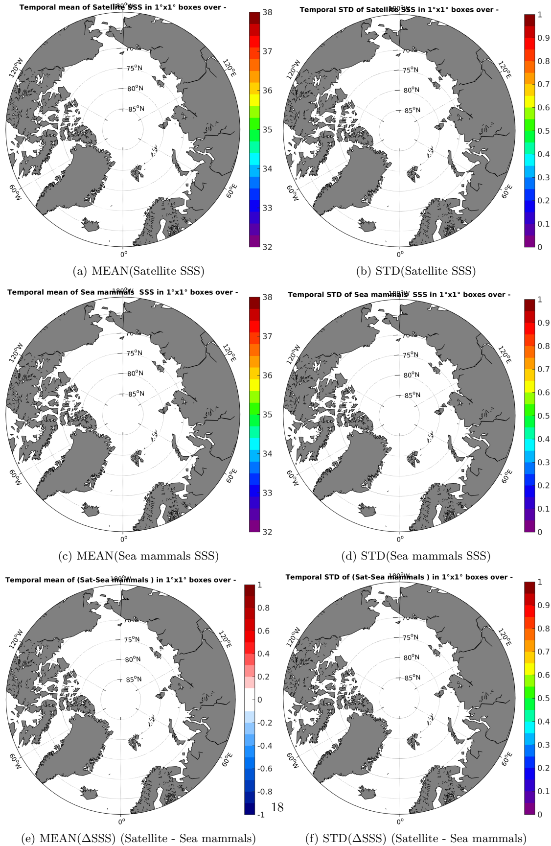
Figure 6: Temporal mean (left) and STD (right) of SSS from AQUARIUS-L2-JPL-V4 (top), Sea mammals (middle), and of \Delta SSS (Satellite - Sea mammals). Only match-up pairs are used to generate these maps.
