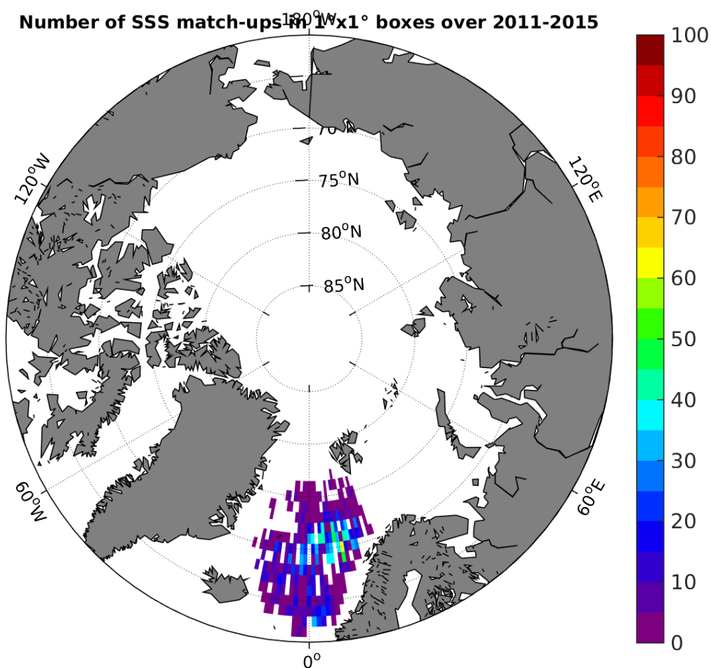
Figure 4: Number of SSS match-ups between Argo SSS and the AQUARIUS-L2-JPL-V4 SSS product for the Arctic Ocean Pi-MEP region over 1^\circ \times 1^\circ boxes and for the full satellite product period.
