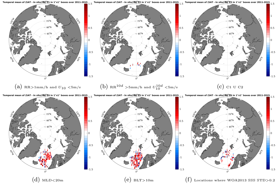
Figure 12: Temporal mean gridded over spatial boxes of size 1^\circ \times 1^\circ of \Delta\text{SSS} (AQUARIUS-L2-JPL-V4 - Argo) for 6 different subdatasets corresponding to: \text{RR} > 1\text{mm/h} and U_{10} < 5\text{m/s} (a), \text{RR}^{10d} > 5\text{mm/h} and U_{10}^{10d} < 5\text{m/s} (b), C1 U C2 (c), \text{MLD} < 20\text{m} (d), \text{BLT} > 10\text{m} (e), Locations where WOA2013 SSS STD > 0.2 (f).
