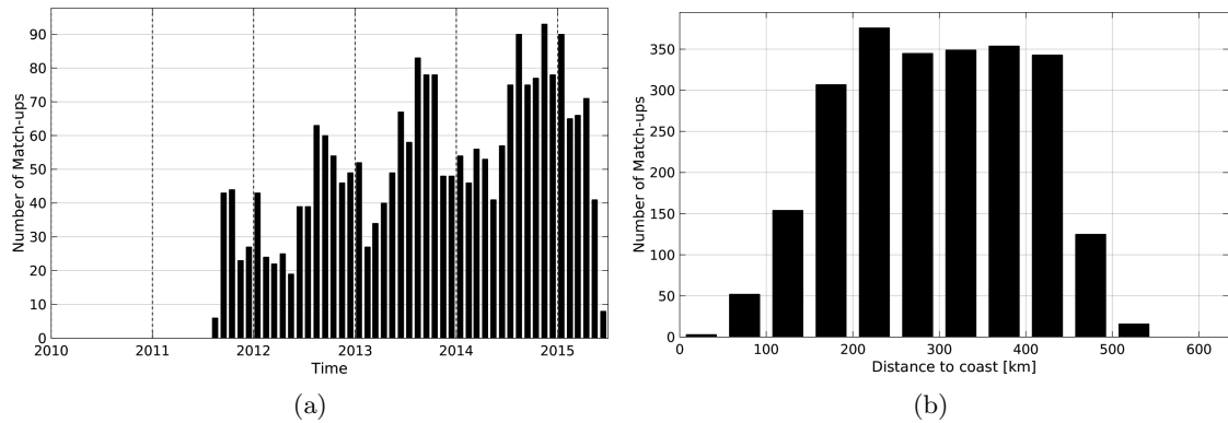
Figure 1: Number of match-ups between Argo and AQUARIUS-L2-JPL-V4 SSS as a function of time (a) and as function of the distance to coast (b) over the Arctic Ocean Pi-MEP region and for the full satellite product period.
