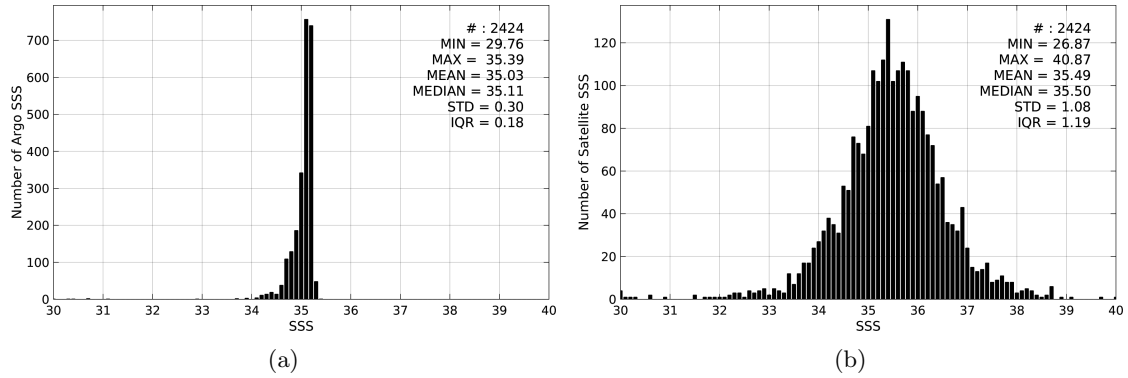
Figure 2: Histograms of SSS from Argo (a) and AQUARIUS-L2-JPL-V4 (b) considering all match-up pairs per bins of 0.1 over the Arctic Ocean Pi-MEP region and for the full satellite product period.
