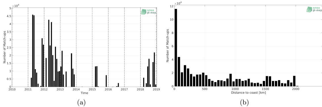
Figure 1: Number of match-ups between TSG (SAMOS) and SMOS and SMAP SSS L4 OI v1 - 7 Days (LOPS) SSS as a function of time (a) and as function of the distance to coast (b) over the Amazon and Orinoco river plumes Pi-MEP region and for the full satellite product period.
