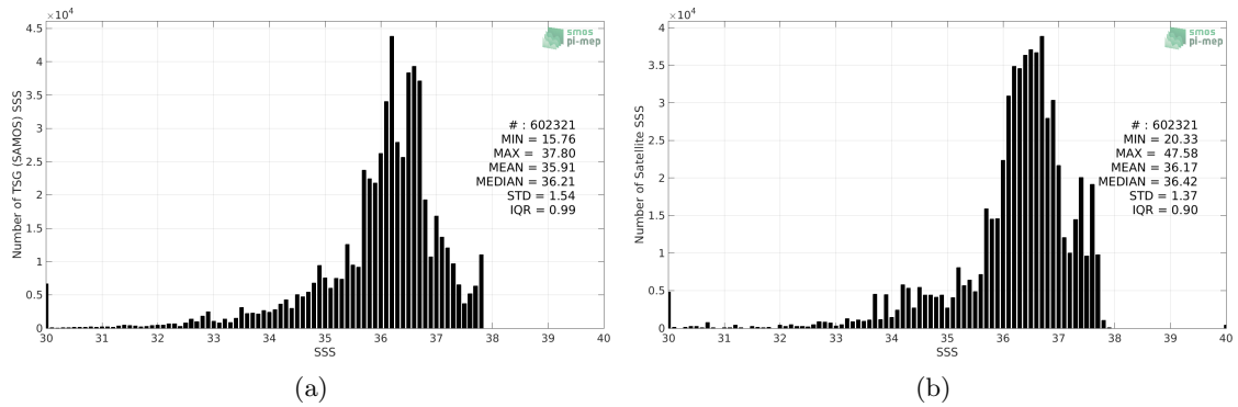
Figure 2: Histograms of SSS from TSG (SAMOS) (a) and SMOS and SMAP SSS L4 OI v1 - 7 Days (LOPS) (b) considering all match-up pairs per bins of 0.1 over the Amazon and Orinoco river plumes Pi-MEP region and for the full satellite product period.
