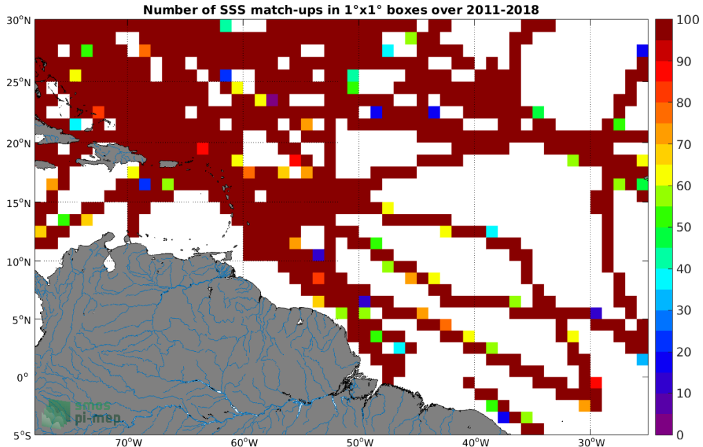
Figure 4: Number of SSS match-ups between TSG (SAMOS) SSS and the SMOS and SMAP SSS L4 OI v1 - 7 Days (LOPS) SSS product for the Amazon and Orinoco river plumes Pi-MEP region over 1^\circ \times 1^\circ boxes and for the full satellite product period.
