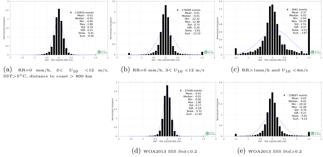
Figure 13: Normalized histogram of \Delta\text{SSS} (SMOS and SMAP SSS L4 OI v1 - 7 Days (LOPS) - TSG (LEGOS-DM)) for 5 different subdatasets corresponding to: RR=0 mm/h, 3 < U_{10} < 12 m/s, SST>5°C, distance to coast > 800 km (a), RR=0 mm/h, 3 < U_{10} < 12 m/s (b), RR>1mm/h and U_{10} < 4 m/s (c), WOA2013 SSS Std<0.2 (d), WOA2013 SSS Std>0.2 (e).
