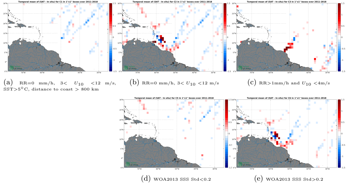
Figure 12: Temporal mean gridded over spatial boxes of size 1^{\circ} \times 1^{\circ} of \Delta\text{SSS} (SMOS and SMAP SSS L4 OI v1 - 7 Days (LOPS) - TSG (LEGOS-DM)) for 5 different subdatasets corresponding to: RR=0 mm/h, 3 < U_{10} < 12 m/s, SST > 5^{\circ}\text{C} , distance to coast > 800 km (a), RR=0 mm/h, 3 < U_{10} < 12 m/s (b), RR > 1 mm/h and U_{10} < 4 m/s (c), WOA2013 SSS Std < 0.2 (d), WOA2013 SSS Std > 0.2 (e).
