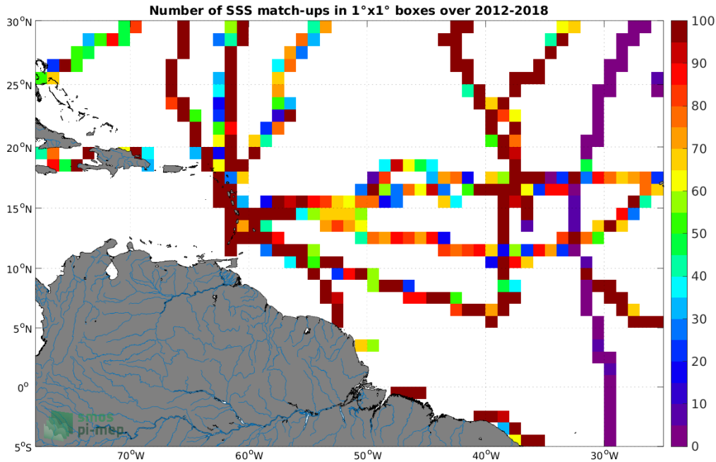
Figure 4: Number of SSS match-ups between TSG (GOSUD-Sailing-ship) SSS and the SMOS and SMAP SSS L4 OI v1 - 7 Days (LOPS) SSS product for the Amazon and Orinoco river plumes Pi-MEP region over 1^{\circ} \times 1^{\circ} boxes and for the full satellite product period.
