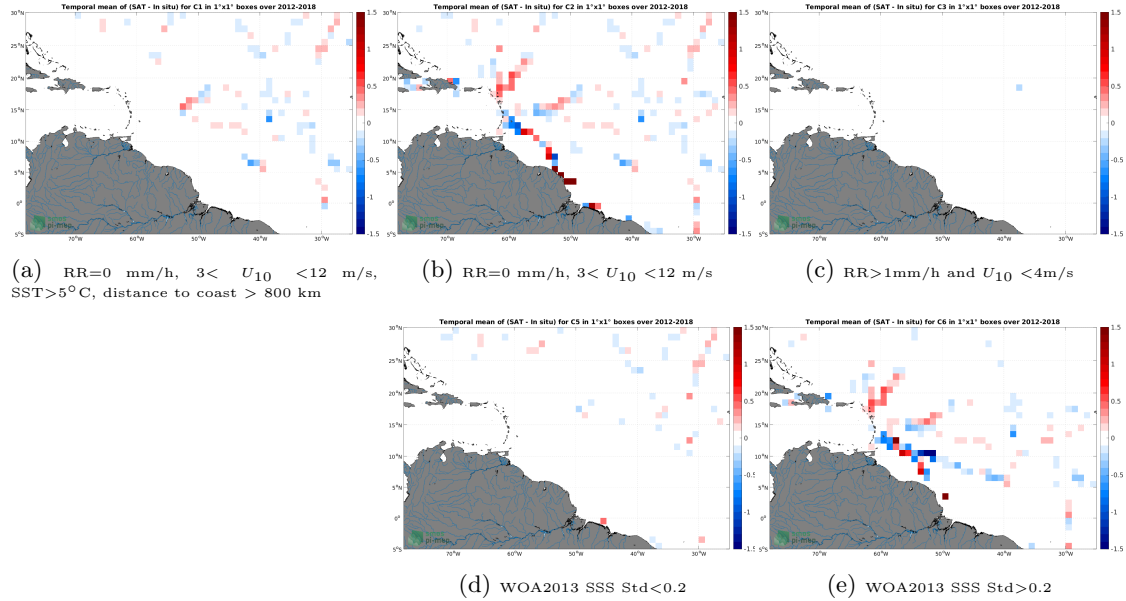
Figure 12: Temporal mean gridded over spatial boxes of size 1^{\circ}\times 1^{\circ} of \Delta SSS (SMOS and SMAP SSS L4 OI v1 - 7 Days (LOPS) - TSG (GOSUD-Sailing-ship)) for 5 different subdatasets corresponding to:RR=0 mm/h, 3 < U_{10} < 12 m/s, SST >5^{\circ}\text{C} , distance to coast > 800 km (a), RR=0 mm/h, 3 < U_{10} < 12 m/s (b), RR >1 mm/h and U_{10} < 4 m/s (c), WOA2013 SSS Std <0.2 (d), WOA2013 SSS Std >0.2 (e).
