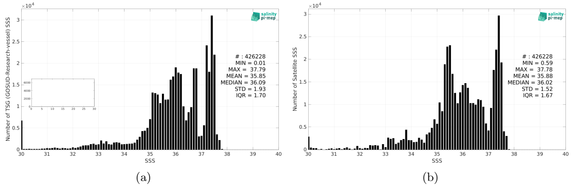
Figure 2: Histograms of SSS from TSG (GOSUD-Research-vessel) (a) and SMOS and SMAP SSS L4 OI v1 - 7 Days (LOPS) (b) considering all match-up pairs per bins of 0.1 over the Amazon and Orinoco river plumes Pi-MEP region and for the full satellite product period.
