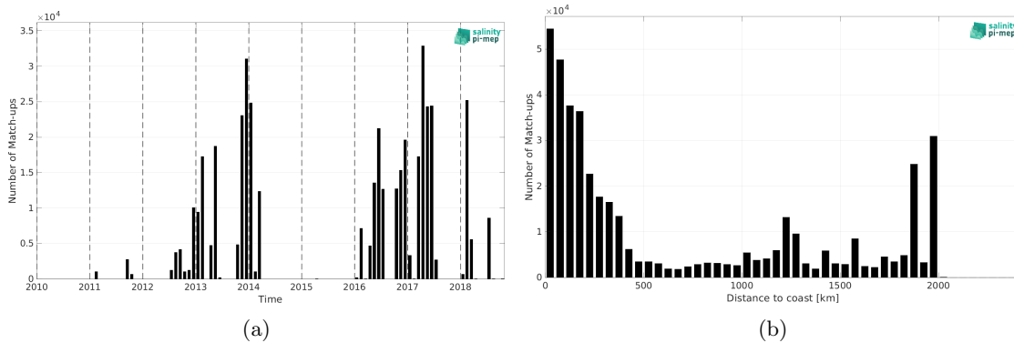
Figure 1: Number of match-ups between TSG (GOSUD-Research-vessel) and SMOS and SMAP SSS L4 OI v1 - 7 Days (LOPS) SSS as a function of time (a) and as function of the distance to coast (b) over the Amazon and Orinoco river plumes Pi-MEP region and for the full satellite product period.
