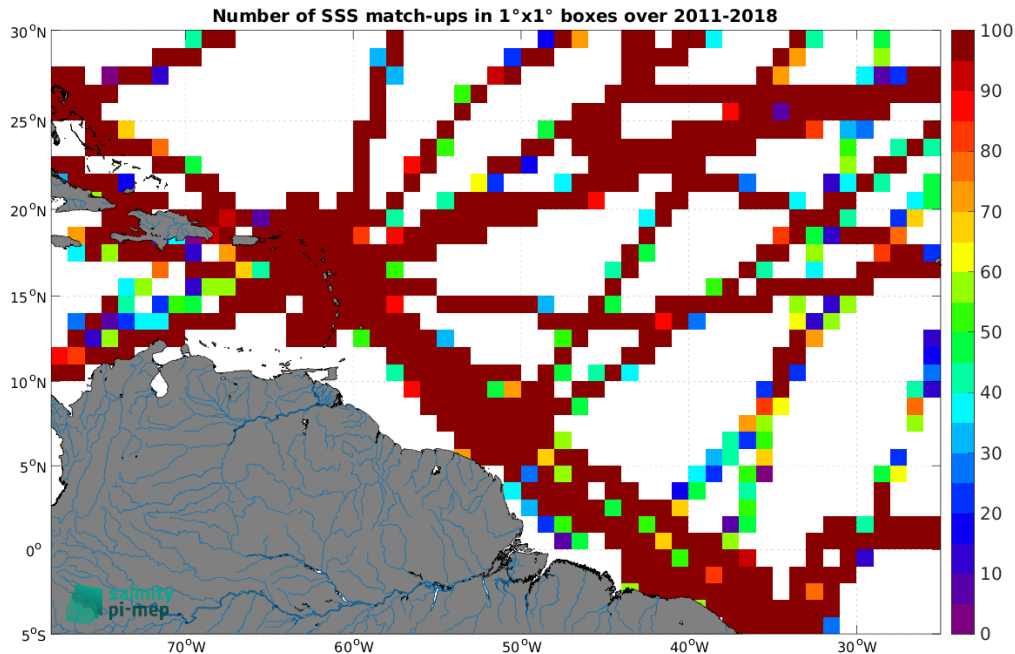
Figure 4: Number of SSS match-ups between TSG (GOSUD-Research-vessel) SSS and the SMOS and SMAP SSS L4 OI v1 - 7 Days (LOPS) SSS product for the Amazon and Orinoco river plumes Pi-MEP region over 1^\circ \times 1^\circ boxes and for the full satellite product period.
