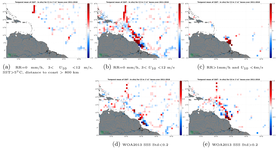
Figure 12: Temporal mean gridded over spatial boxes of size 1^{\circ}\times 1^{\circ} of \Delta SSS (SMOS and SMAP SSS L4 OI v1 - 7 Days (LOPS) - TSG (GOSUD-Research-vessel)) for 5 different subdatasets corresponding to:RR=0 mm/h, 3 < U_{10} < 12 m/s, SST >5^{\circ}\text{C} , distance to coast > 800 km (a), RR=0 mm/h, 3 < U_{10} < 12 m/s (b), RR >1 mm/h and U_{10} < 4 m/s (c), WOA2013 SSS Std <0.2 (d), WOA2013 SSS Std >0.2 (e).
