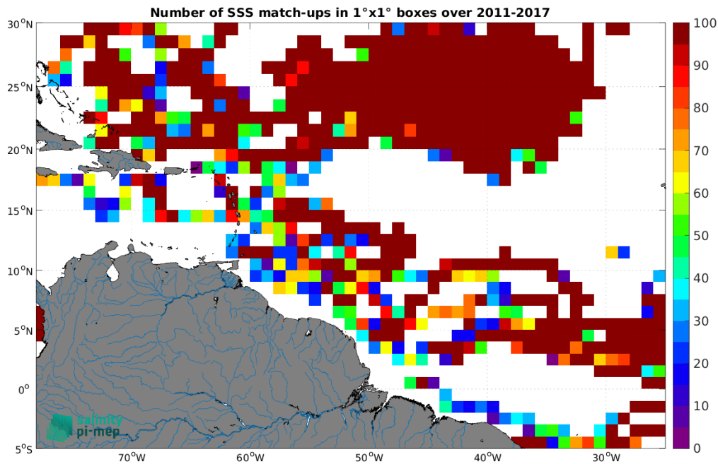
Figure 3: Number of SSS match-ups between Surface drifters SSS and the SMOS and SMAP SSS L4 OI v1 - 7 Days (LOPS) SSS product for the Amazon and Orinoco river plumes Pi-MEP region over 1^{\circ} \times 1^{\circ} boxes and for the full satellite product period.
