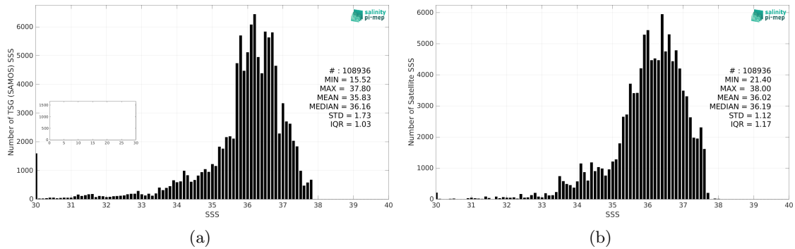
Figure 2: Histograms of SSS from TSG (SAMOS) (a) and SMOS SSS L4 v1 - Weekly (CMEMS-CNR) (b) considering all match-up pairs per bins of 0.1 over the Amazon and Orinoco river plumes Pi-MEP region and for the full satellite product period.
