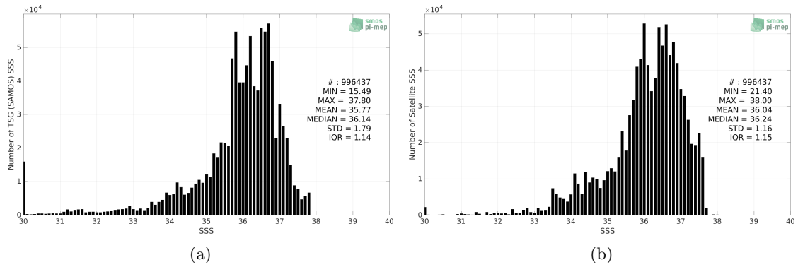
Figure 2: Histograms of SSS from TSG (SAMOS) (a) and SMOS SSS L4 v1 - Weekly (CMEMS-CNR) (b) considering all match-up pairs per bins of 0.1 over the Amazon and Orinoco river plumes Pi-MEP region and for the full satellite product period.
