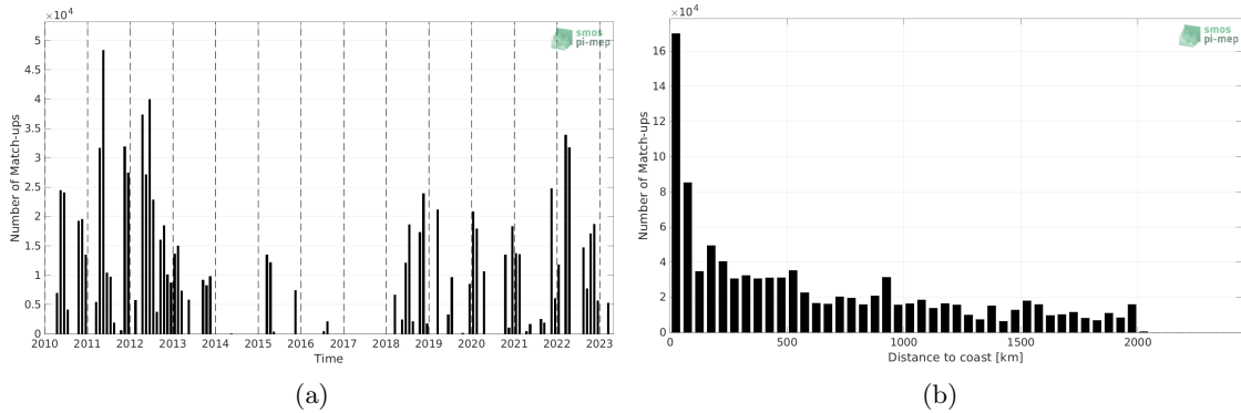
Figure 1: Number of match-ups between TSG (SAMOS) and SMOS SSS L4 v1 - Weekly (CMEMS-CNR) SSS as a function of time (a) and as function of the distance to coast (b) over the Amazon and Orinoco river plumes Pi-MEP region and for the full satellite product period.
