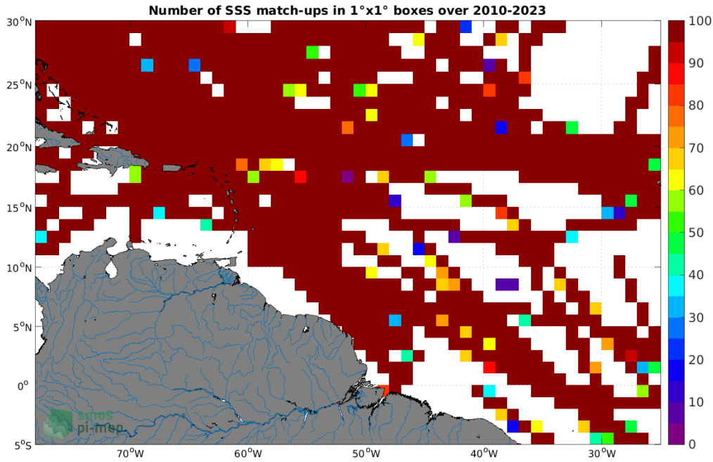
Figure 4: Number of SSS match-ups between TSG (SAMOS) SSS and the SMOS SSS L4 v1 - Weekly (CMEMS-CNR) SSS product for the Amazon and Orinoco river plumes Pi-MEP region over 1^\circ \times 1^\circ boxes and for the full satellite product period.
