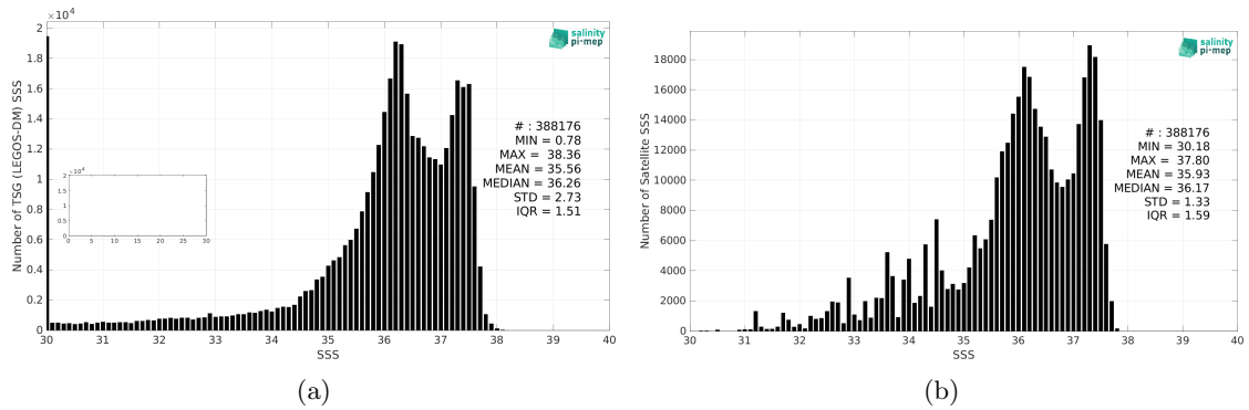
Figure 2: Histograms of SSS from TSG (LEGOS-DM) (a) and SMOS SSS L4 v1 - Weekly (CMEMS-CNR) (b) considering all match-up pairs per bins of 0.1 over the Amazon and Orinoco river plumes Pi-MEP region and for the full satellite product period.
