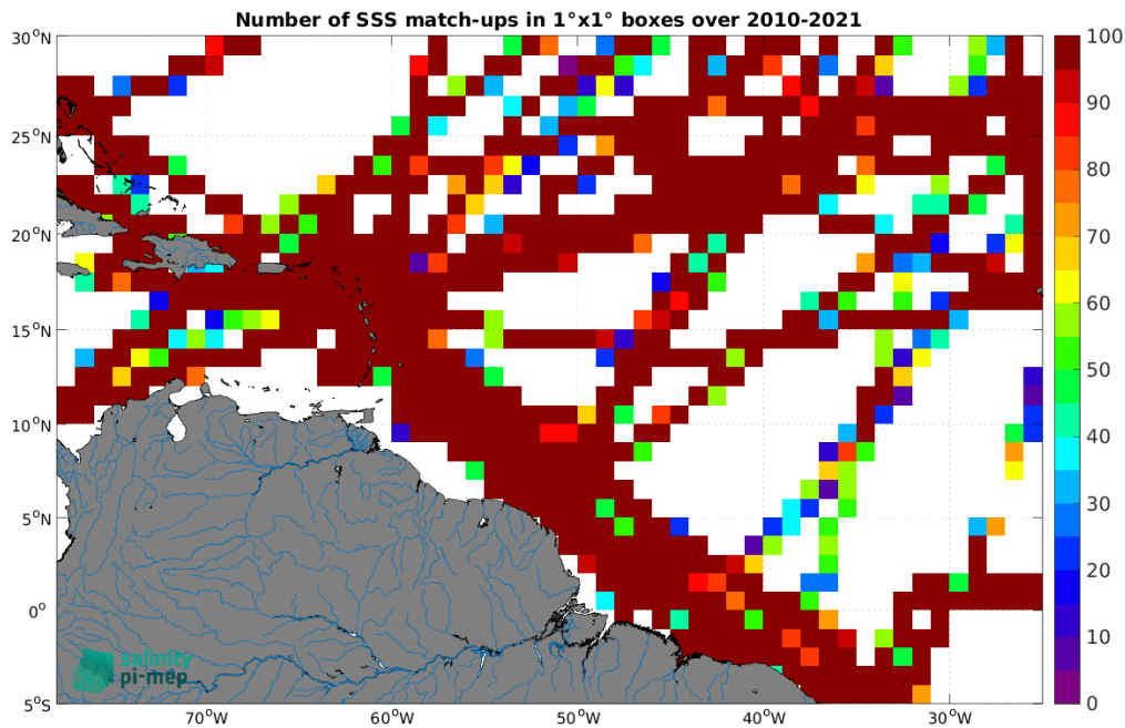
Figure 4: Number of SSS match-ups between TSG (GOSUD-Research-vessel) SSS and the SMOS SSS L4 v1 - Weekly (CMEMS-CNR) SSS product for the Amazon and Orinoco river plumes Pi-MEP region over 1^{\circ} \times 1^{\circ} boxes and for the full satellite product period.
