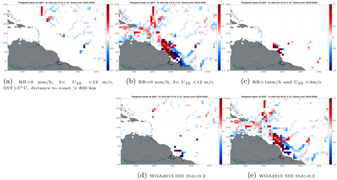
Figure 12: Temporal mean gridded over spatial boxes of size 1^{\circ}\times 1^{\circ} of \Delta SSS (SMOS SSS L4 v1 - Weekly (CMEMS-CNR) - TSG (GOSUD-Research-vessel)) for 5 different subdatasets corresponding to:RR=0 mm/h, 3 < U_{10} < 12 m/s, SST >5^{\circ}\text{C} , distance to coast > 800 km (a), RR=0 mm/h, 3 < U_{10} < 12 m/s (b), RR >1 mm/h and U_{10} < 4 m/s (c), WOA2013 SSS Std <0.2 (d), WOA2013 SSS Std >0.2 (e).
