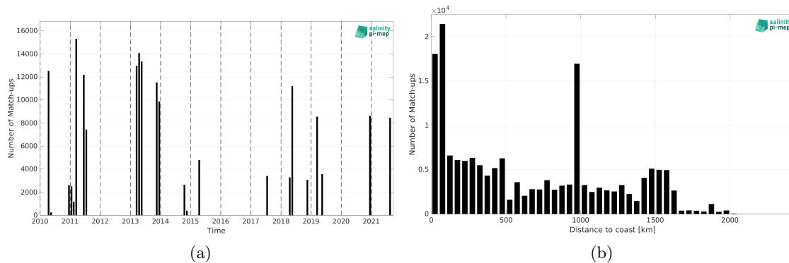
Figure 1: Number of match-ups between TSG (CSIC-UTM) and SMOS SSS L4 v1 - Weekly (CMEMS-CNR) SSS as a function of time (a) and as function of the distance to coast (b) over the Amazon and Orinoco river plumes Pi-MEP region and for the full satellite product period.
