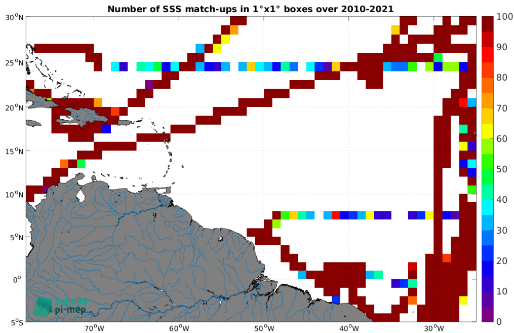
Figure 4: Number of SSS match-ups between TSG (CSIC-UTM) SSS and the SMOS SSS L4 v1 - Weekly (CMEMS-CNR) SSS product for the Amazon and Orinoco river plumes Pi-MEP region over 1^\circ \times 1^\circ boxes and for the full satellite product period.
