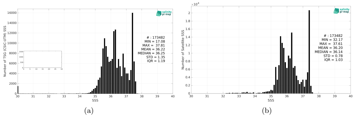
Figure 2: Histograms of SSS from TSG (CSIC-UTM) (a) and SMOS SSS L4 v1 - Weekly (CMEMS-CNR) (b) considering all match-up pairs per bins of 0.1 over the Amazon and Orinoco river plumes Pi-MEP region and for the full satellite product period.
