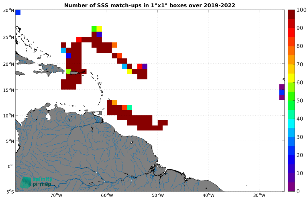
Figure 4: Number of SSS match-ups between Saildrone SSS and the SMOS SSS L4 v1 - Weekly (CMEMS-CNR) SSS product for the Amazon and Orinoco river plumes Pi-MEP region over 1^\circ \times 1^\circ boxes and for the full satellite product period.
