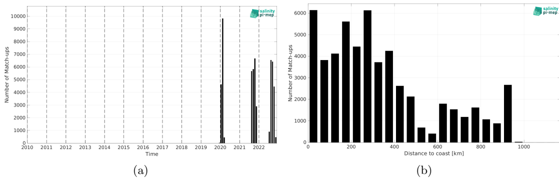
Figure 1: Number of match-ups between Saildrone and SMOS SSS L4 v1 - Weekly (CMEMS-CNR) SSS as a function of time (a) and as function of the distance to coast (b) over the Amazon and Orinoco river plumes Pi-MEP region and for the full satellite product period.
