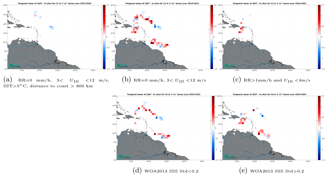
Figure 12: Temporal mean gridded over spatial boxes of size 1^\circ \times 1^\circ of \Delta SSS (SMOS SSS L4 v1 - Weekly (CMEMS-CNR) - Sailldrone) for 5 different subdatasets corresponding to:RR=0 mm/h, 3 < U_{10} < 12 m/s, SST >5^\circ\text{C} , distance to coast > 800 km (a), RR=0 mm/h, 3 < U_{10} < 12 m/s (b), RR >1 mm/h and U_{10} < 4 m/s (c), WOA2013 SSS Std <0.2 (d), WOA2013 SSS Std >0.2 (e).
