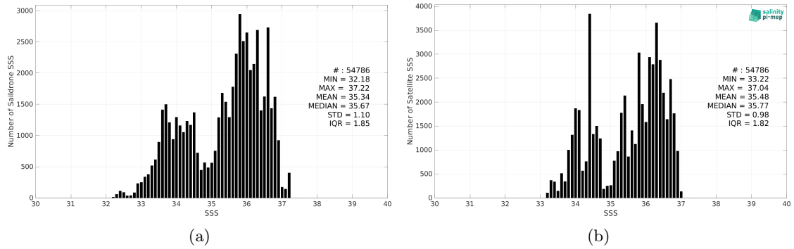
Figure 2: Histograms of SSS from Sailability (a) and SMOS SSS L4 v1 - Weekly (CMEMS-CNR) (b) considering all match-up pairs per bins of 0.1 over the Amazon and Orinoco river plumes Pi-MEP region and for the full satellite product period.
