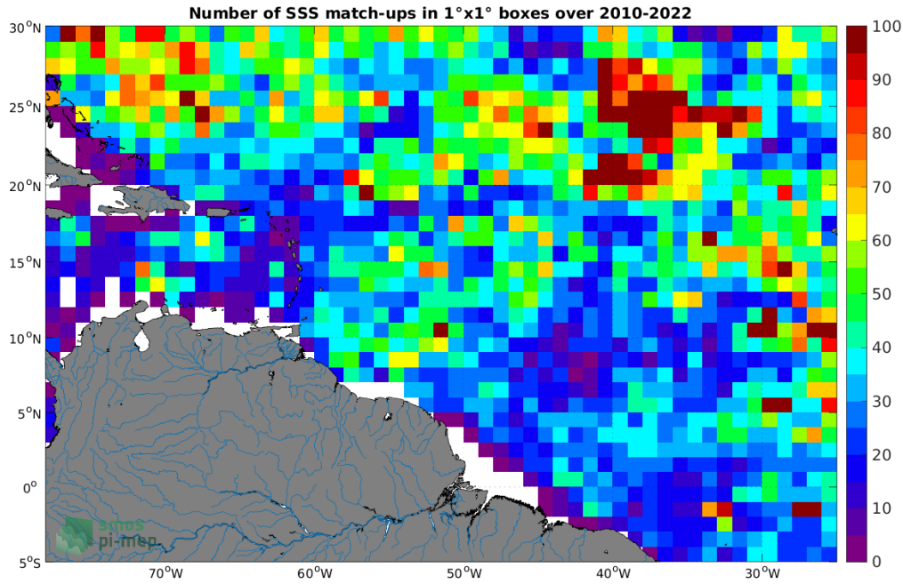
Figure 4: Number of SSS match-ups between Argo SSS and the SMOS SSS L4 v1 - Weekly (CMEMS-CNR) SSS product for the Amazon and Orinoco river plumes Pi-MEP region over 1^\circ \times 1^\circ boxes and for the full satellite product period.
