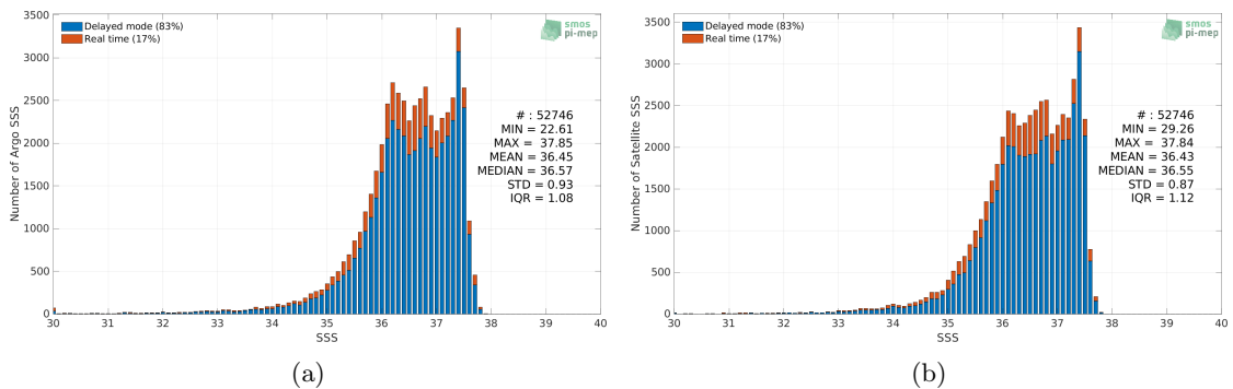
Figure 2: Histograms of SSS from Argo (a) and SMOS SSS L4 v1 - Weekly (CMEMS-CNR) (b) considering all match-up pairs per bins of 0.1 over the Amazon and Orinoco river plumes Pi-MEP region and for the full satellite product period.
