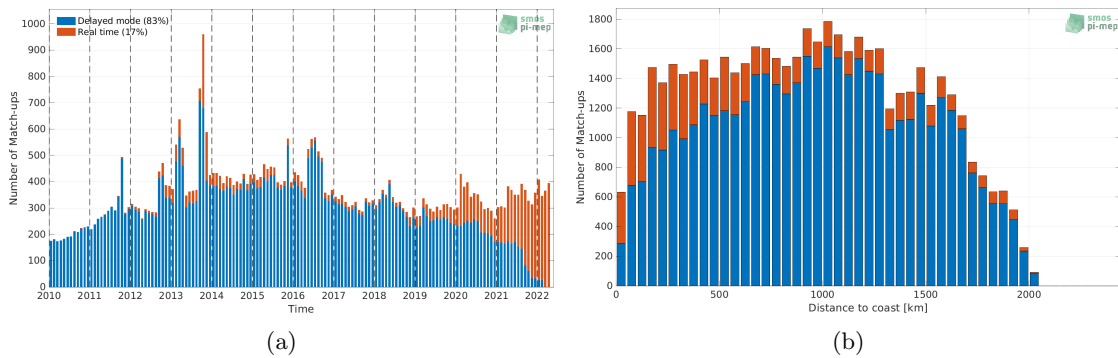
Figure 1: Number of match-ups between Argo and SMOS SSS L4 v1 - Weekly (CMEMS-CNR) SSS as a function of time (a) and as function of the distance to coast (b) over the Amazon and Orinoco river plumes Pi-MEP region and for the full satellite product period.
