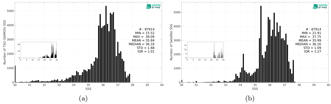
Figure 3: Histograms of SSS from TSG (SAMOS) (a) and SMOS SSS L4 v1 - Monthly (CMEMS-CNR) (b) considering all match-up pairs per bins of 0.1 over the Amazon and Orinoco river plumes Pi-MEP region and for the full satellite product period.
