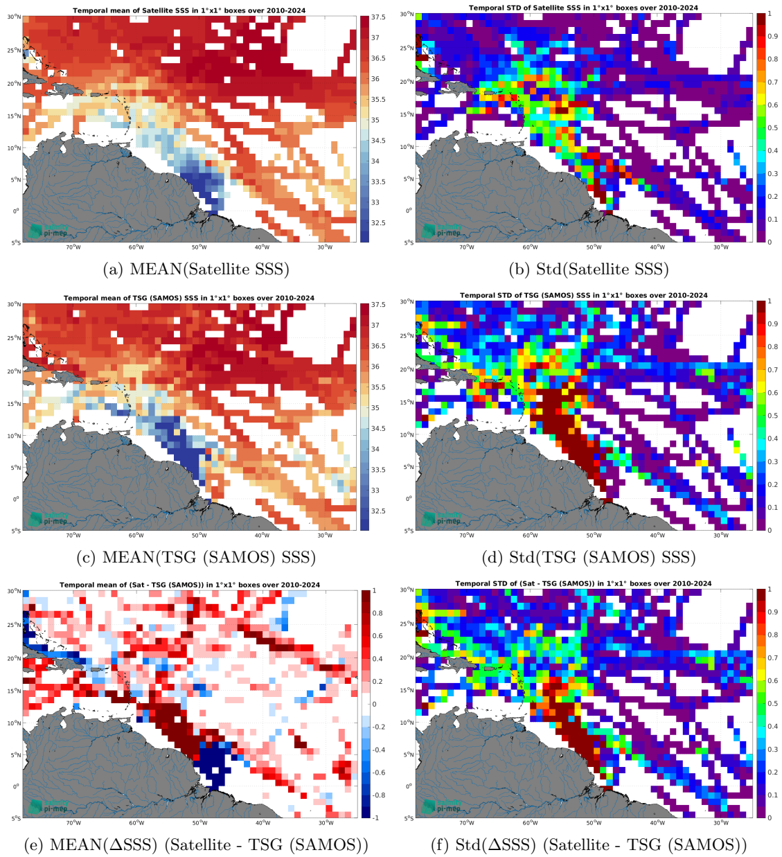
Figure 7: Temporal mean (left) and Std (right) of SSS from SMOS SSS L4 v1 - Monthly (CMEMS-CNR) (top), TSG (SAMOS) (middle), and of \Delta SSS (Satellite - TSG (SAMOS)). Only match-up pairs are used to generate these maps.
