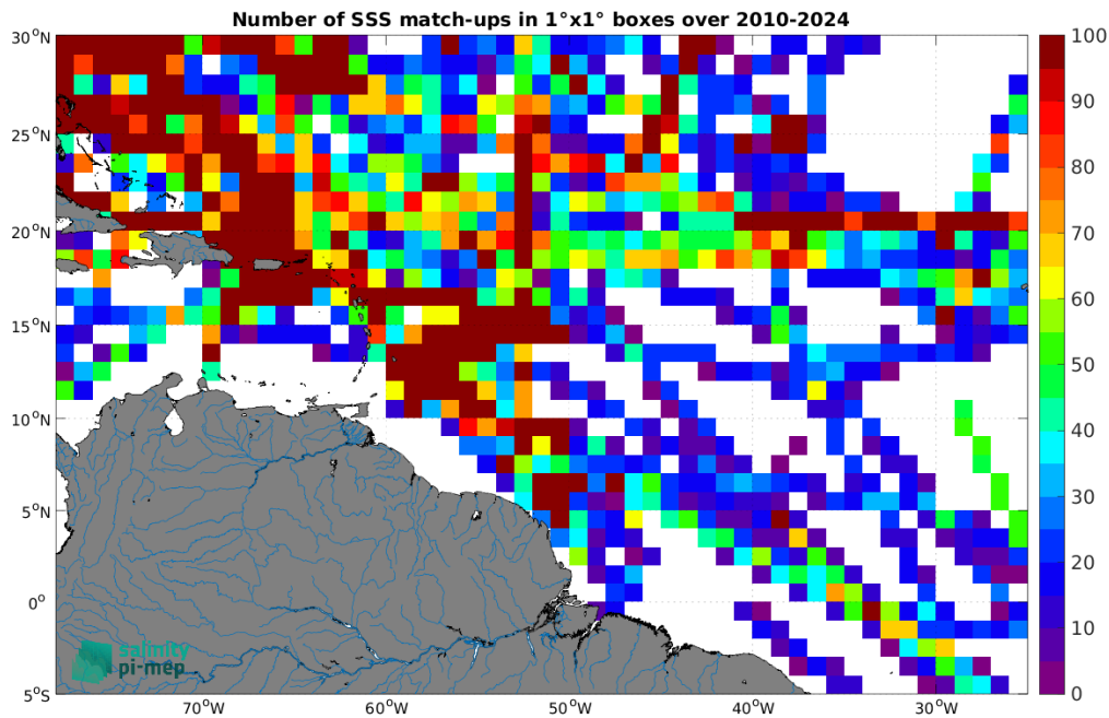
Figure 5: Number of SSS match-ups between TSG (SAMOS) SSS and the SMOS SSS L4 v1 - Monthly (CMEMS-CNR) SSS product for the Amazon and Orinoco river plumes Pi-MEP region over 1^\circ \times 1^\circ boxes and for the full satellite product period.
