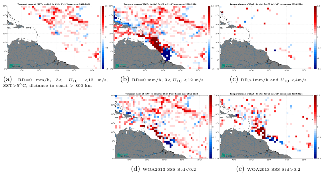
Figure 14: Temporal mean gridded over spatial boxes of size 1^\circ \times 1^\circ of \Delta SSS (SMOS SSS L4 v1 - Monthly (CMEMS-CNR) - TSG (SAMOS)) for 5 different subdatasets corresponding to:RR=0 mm/h, 3 < U_{10} < 12 m/s, SST >5^\circ\text{C} , distance to coast > 800 km (a), RR=0 mm/h, 3 < U_{10} < 12 m/s (b), RR >1 mm/h and U_{10} < 4 m/s (c), WOA2013 SSS Std <0.2 (d), WOA2013 SSS Std >0.2 (e).
