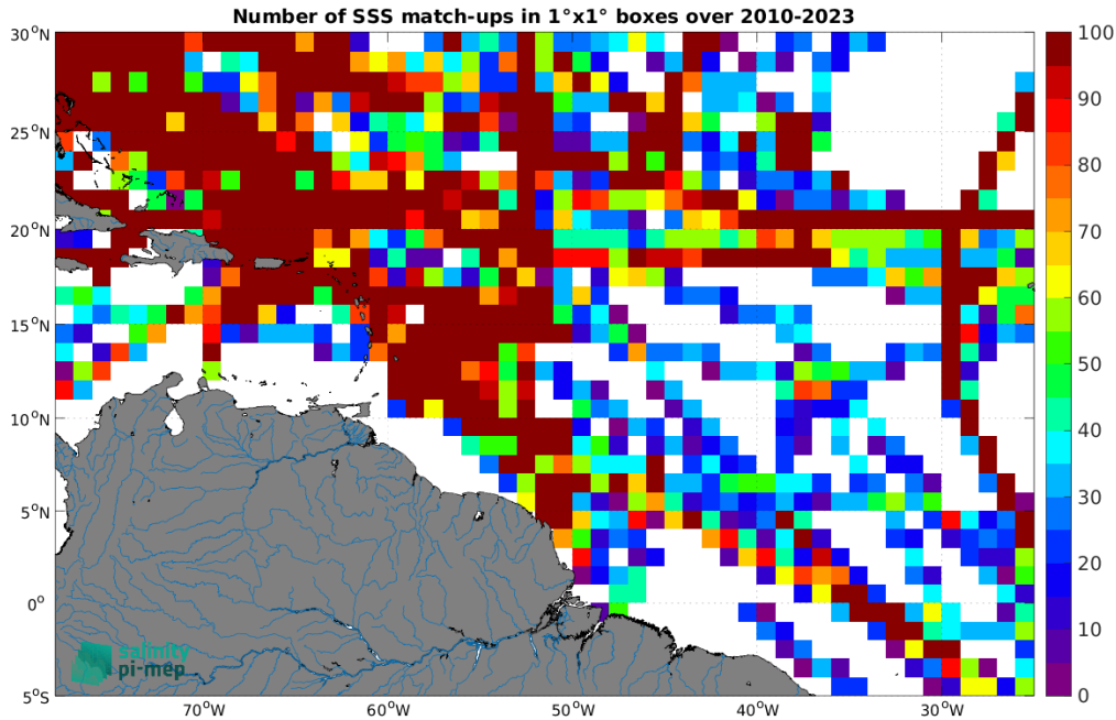
Figure 4: Number of SSS match-ups between TSG (SAMOS) SSS and the SMOS SSS L4 v1 - Monthly (CMEMS-CNR) SSS product for the Amazon and Orinoco river plumes Pi-MEP region over 1^\circ \times 1^\circ boxes and for the full satellite product period.
