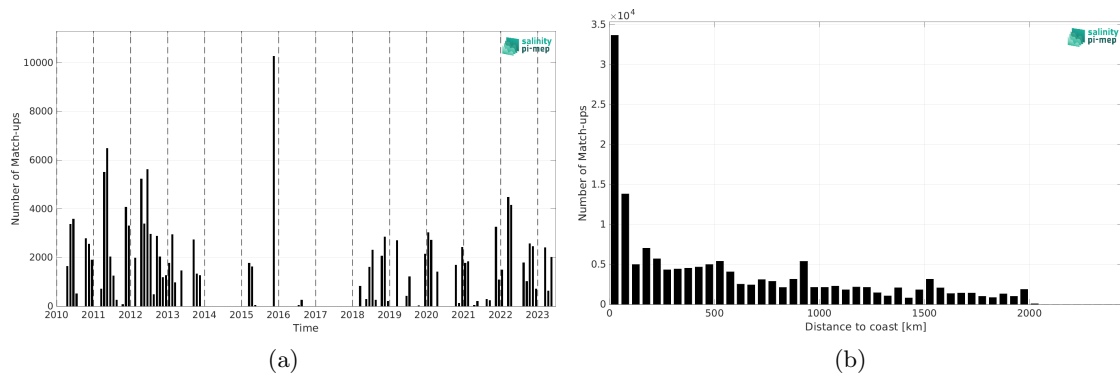
Figure 1: Number of match-ups between TSG (SAMOS) and SMOS SSS L4 v1 - Monthly (CMEMS-CNR) SSS as a function of time (a) and as function of the distance to coast (b) over the Amazon and Orinoco river plumes Pi-MEP region and for the full satellite product period.
