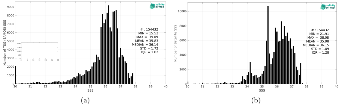
Figure 2: Histograms of SSS from TSG (SAMOS) (a) and SMOS SSS L4 v1 - Monthly (CMEMS-CNR) (b) considering all match-up pairs per bins of 0.1 over the Amazon and Orinoco river plumes Pi-MEP region and for the full satellite product period.
