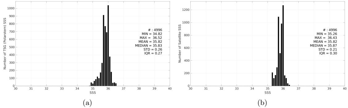
Figure 3: Histograms of SSS from TSG (Polarstern) (a) and SMOS SSS L4 v1 - Monthly (CMEMS-CNR) (b) considering all match-up pairs per bins of 0.1 over the Amazon and Orinoco river plumes Pi-MEP region and for the full satellite product period.
