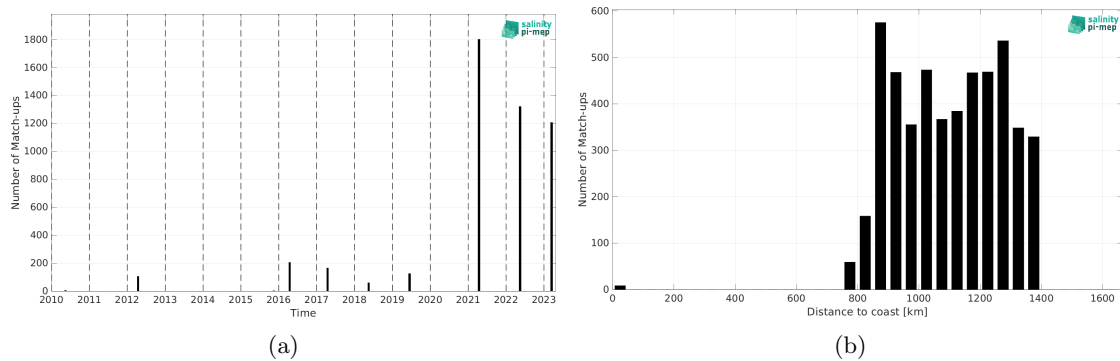
Figure 2: Number of match-ups between TSG (Polarstern) and SMOS SSS L4 v1 - Monthly (CMEMS-CNR) SSS as a function of time (a) and as function of the distance to coast (b) over the Amazon and Orinoco river plumes Pi-MEP region and for the full satellite product period.
