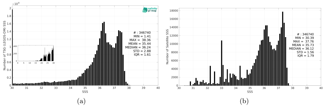
Figure 3: Histograms of SSS from TSG (LEGOS-DM) (a) and SMOS SSS L4 v1 - Monthly (CMEMS-CNR) (b) considering all match-up pairs per bins of 0.1 over the Amazon and Orinoco river plumes Pi-MEP region and for the full satellite product period.
