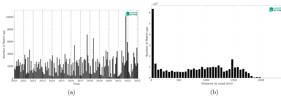
Figure 2: Number of match-ups between TSG (LEGOS-DM) and SMOS SSS L4 v1 - Monthly (CMEMS-CNR) SSS as a function of time (a) and as function of the distance to coast (b) over the Amazon and Orinoco river plumes Pi-MEP region and for the full satellite product period.
