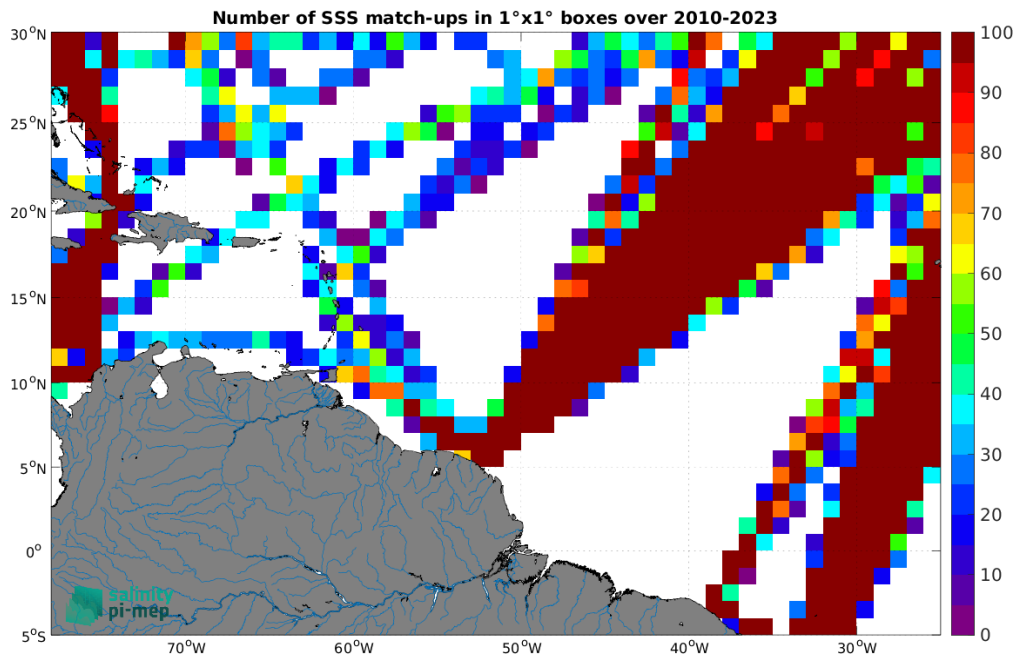
Figure 5: Number of SSS match-ups between TSG (LEGOS-DM) SSS and the SMOS SSS L4 v1 - Monthly (CMEMS-CNR) SSS product for the Amazon and Orinoco river plumes Pi-MEP region over 1^{\circ} \times 1^{\circ} boxes and for the full satellite product period.
