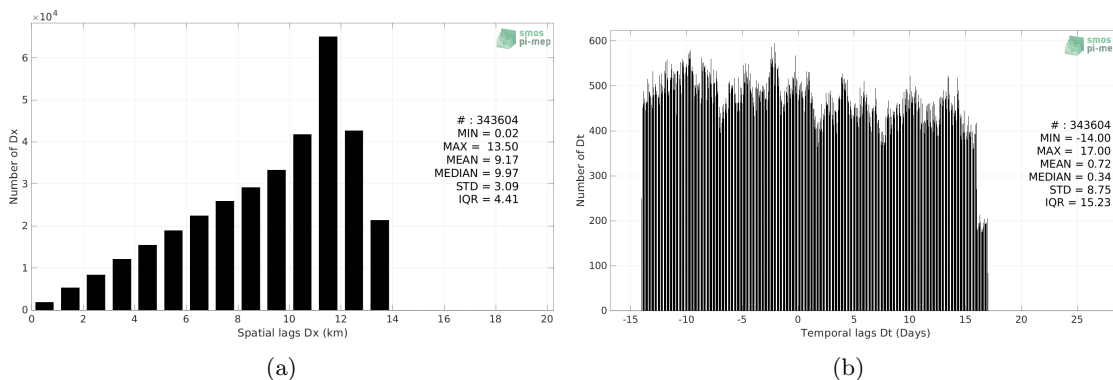
Figure 5: Histograms of the spatial (a) and temporal (b) lags between the location/time of the TSG (LEGOS-DM) measurement and the date of the corresponding SMOS SSS L4 v1 - Monthly (CMEMS-CNR) SSS pixel.
