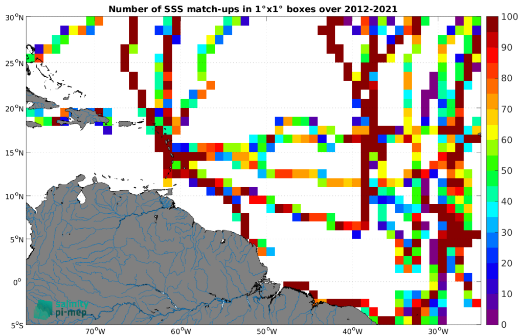
Figure 5: Number of SSS match-ups between TSG (GOSUD-Sailing-ship) SSS and the SMOS SSS L4 v1 - Monthly (CMEMS-CNR) SSS product for the Amazon and Orinoco river plumes Pi-MEP region over 1^\circ \times 1^\circ boxes and for the full satellite product period.
