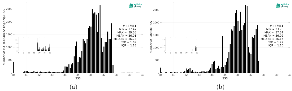
Figure 3: Histograms of SSS from TSG (GOSUD-Sailing-ship) (a) and SMOS SSS L4 v1 - Monthly (CMEMS-CNR) (b) considering all match-up pairs per bins of 0.1 over the Amazon and Orinoco river plumes Pi-MEP region and for the full satellite product period.
