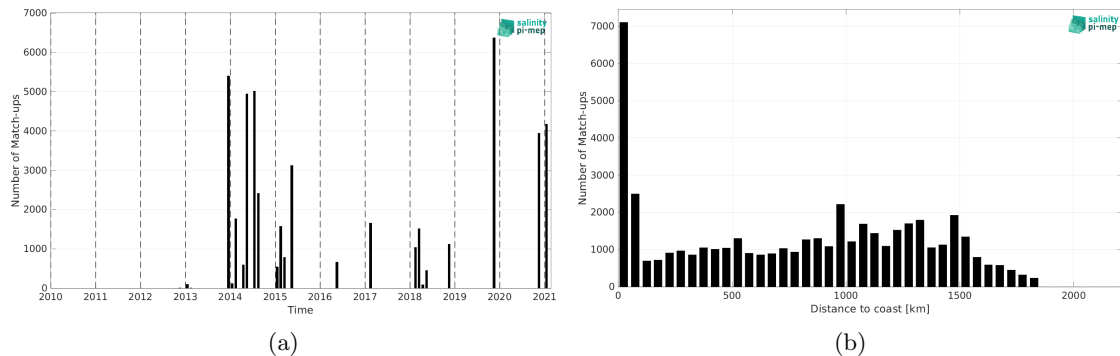
Figure 2: Number of match-ups between TSG (GOSUD-Sailing-ship) and SMOS SSS L4 v1 - Monthly (CMEMS-CNR) SSS as a function of time (a) and as function of the distance to coast (b) over the Amazon and Orinoco river plumes Pi-MEP region and for the full satellite product period.
