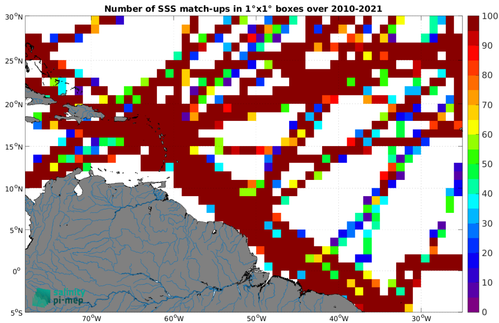
Figure 5: Number of SSS match-ups between TSG (GOSUD-Research-vessel) SSS and the SMOS SSS L4 v1 - Monthly (CMEMS-CNR) SSS product for the Amazon and Orinoco river plumes Pi-MEP region over 1^\circ \times 1^\circ boxes and for the full satellite product period.
