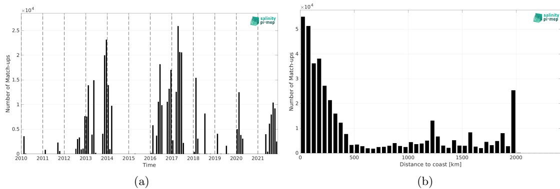
Figure 2: Number of match-ups between TSG (GOSUD-Research-vessel) and SMOS SSS L4 v1 - Monthly (CMEMS-CNR) SSS as a function of time (a) and as function of the distance to coast (b) over the Amazon and Orinoco river plumes Pi-MEP region and for the full satellite product period.
