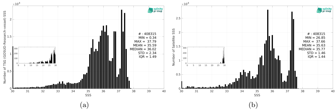
Figure 3: Histograms of SSS from TSG (GOSUD-Research-vessel) (a) and SMOS SSS L4 v1 - Monthly (CMEMS-CNR) (b) considering all match-up pairs per bins of 0.1 over the Amazon and Orinoco river plumes Pi-MEP region and for the full satellite product period.
