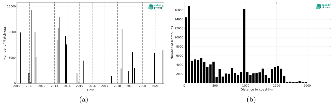
Figure 2: Number of match-ups between TSG (CSIC-UTM) and SMOS SSS L4 v1 - Monthly (CMEMS-CNR) SSS as a function of time (a) and as function of the distance to coast (b) over the Amazon and Orinoco river plumes Pi-MEP region and for the full satellite product period.
