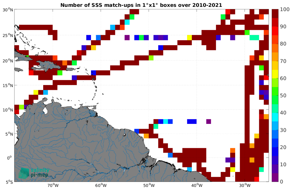
Figure 5: Number of SSS match-ups between TSG (CSIC-UTM) SSS and the SMOS SSS L4 v1 - Monthly (CMEMS-CNR) SSS product for the Amazon and Orinoco river plumes Pi-MEP region over 1^\circ \times 1^\circ boxes and for the full satellite product period.
