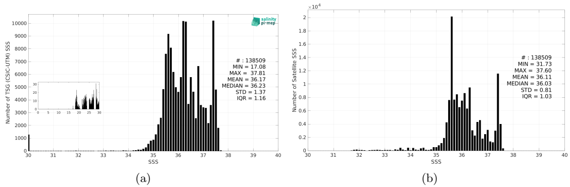
Figure 3: Histograms of SSS from TSG (CSIC-UTM) (a) and SMOS SSS L4 v1 - Monthly (CMEMS-CNR) (b) considering all match-up pairs per bins of 0.1 over the Amazon and Orinoco river plumes Pi-MEP region and for the full satellite product period.
