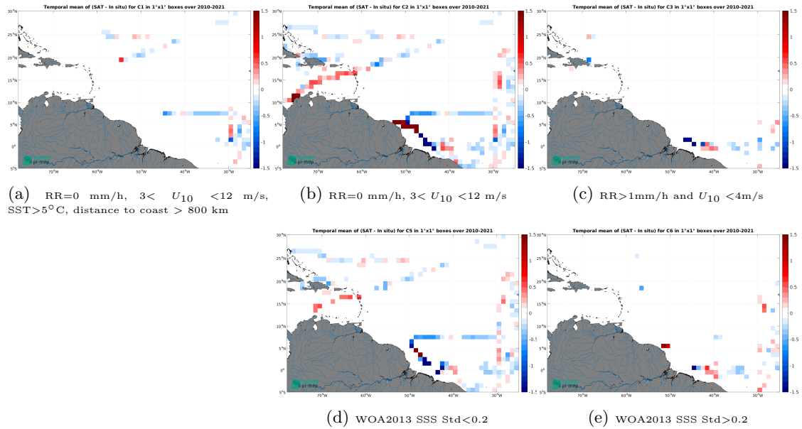
Figure 12: Temporal mean gridded over spatial boxes of size 1^\circ \times 1^\circ of \Delta SSS (SMOS SSS L4 v1 - Monthly (CMEMS-CNR) - TSG (CSIC-UTM)) for 5 different subdatasets corresponding to:RR=0 mm/h, 3 < U_{10} < 12 m/s, SST >5^\circ C, distance to coast > 800 km (a), RR=0 mm/h, 3 < U_{10} < 12 m/s (b), RR >1 mm/h and U_{10} < 4 m/s (c), WOA2013 SSS Std <0.2 (d), WOA2013 SSS Std >0.2 (e).
