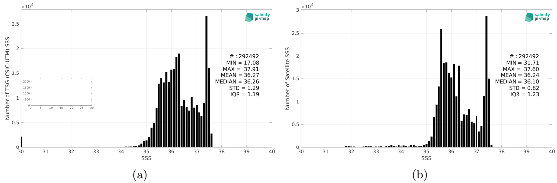
Figure 2: Histograms of SSS from TSG (CSIC-UTM) (a) and SMOS SSS L4 v1 - Monthly (CMEMS-CNR) (b) considering all match-up pairs per bins of 0.1 over the Amazon and Orinoco river plumes Pi-MEP region and for the full satellite product period.
