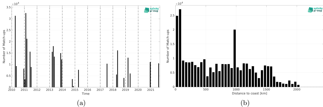
Figure 1: Number of match-ups between TSG (CSIC-UTM) and SMOS SSS L4 v1 - Monthly (CMEMS-CNR) SSS as a function of time (a) and as function of the distance to coast (b) over the Amazon and Orinoco river plumes Pi-MEP region and for the full satellite product period.
