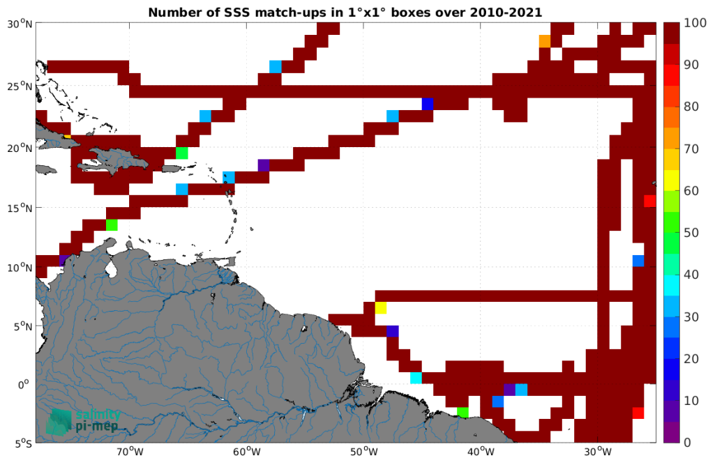
Figure 4: Number of SSS match-ups between TSG (CSIC-UTM) SSS and the SMOS SSS L4 v1 - Monthly (CMEMS-CNR) SSS product for the Amazon and Orinoco river plumes Pi-MEP region over 1^{\circ} \times 1^{\circ} boxes and for the full satellite product period.
