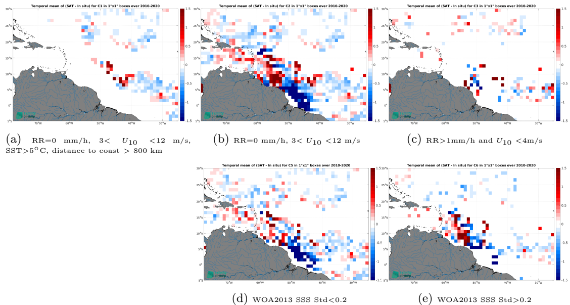
Figure 13: Temporal mean gridded over spatial boxes of size 1^\circ \times 1^\circ of \Delta\text{SSS} (SMOS SSS L4 v1 - Monthly (CMEMS-CNR) - Surface drifters) for 5 different subdatasets corresponding to:RR=0 mm/h, 3 < U_{10} < 12 m/s, SST >5^\circ\text{C} , distance to coast > 800 km (a), RR=0 mm/h, 3 < U_{10} < 12 m/s (b), RR >1 mm/h and U_{10} < 4 m/s (c), WOA2013 SSS Std <0.2 (d), WOA2013 SSS Std >0.2 (e).
