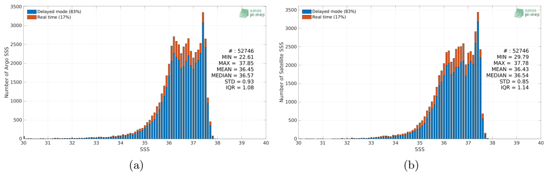
Figure 2: Histograms of SSS from Argo (a) and SMOS SSS L4 v1 - Monthly (CMEMS-CNR) (b) considering all match-up pairs per bins of 0.1 over the Amazon and Orinoco river plumes Pi-MEP region and for the full satellite product period.
