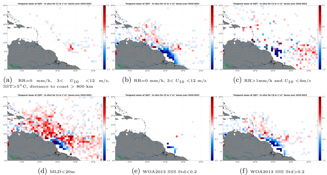
Figure 12: Temporal mean gridded over spatial boxes of size 1^\circ \times 1^\circ of \Delta SSS (SMOS SSS L4 v1 - Monthly (CMEMS-CNR) - Argo) for 6 different subdatasets corresponding to: RR=0 mm/h, 3 < U_{10} < 12 m/s, SST > 5^\circ\text{C} , distance to coast > 800 km (a), RR=0 mm/h, 3 < U_{10} < 12 m/s (b), RR > 1 mm/h and U_{10} < 4 m/s (c), MLD < 20 m (d), WOA2013 SSS Std < 0.2 (e), WOA2013 SSS Std > 0.2 (f).
