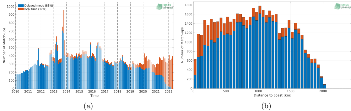
Figure 1: Number of match-ups between Argo and SMOS SSS L4 v1 - Monthly (CMEMS-CNR) SSS as a function of time (a) and as function of the distance to coast (b) over the Amazon and Orinoco river plumes Pi-MEP region and for the full satellite product period.
