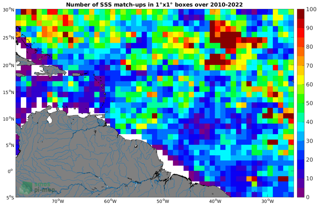
Figure 4: Number of SSS match-ups between Argo SSS and the SMOS SSS L4 v1 - Monthly (CMEMS-CNR) SSS product for the Amazon and Orinoco river plumes Pi-MEP region over 1^\circ \times 1^\circ boxes and for the full satellite product period.
