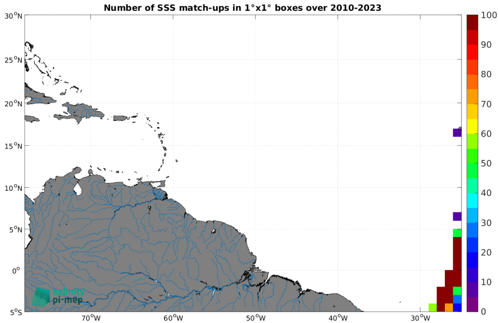
Figure 5: Number of SSS match-ups between TSG (Polarstern) SSS and the SMOS SSS L4 v1 - Daily (CMEMS-CNR) SSS product for the Amazon and Orinoco river plumes Pi-MEP region over 1°×1° boxes and for the full satellite product period.
