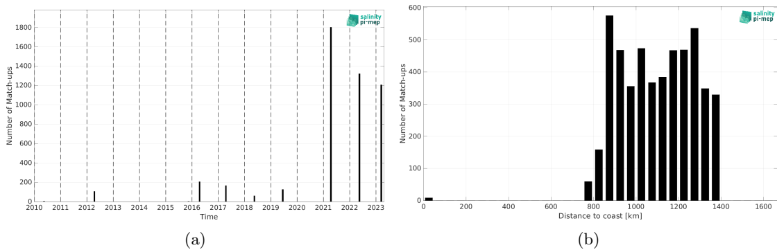
Figure 2: Number of match-ups between TSG (Polarstern) and SMOS SSS L4 v1 - Daily (CMEMS-CNR) SSS as a function of time (a) and as function of the distance to coast (b) over the Amazon and Orinoco river plumes Pi-MEP region and for the full satellite product period.
