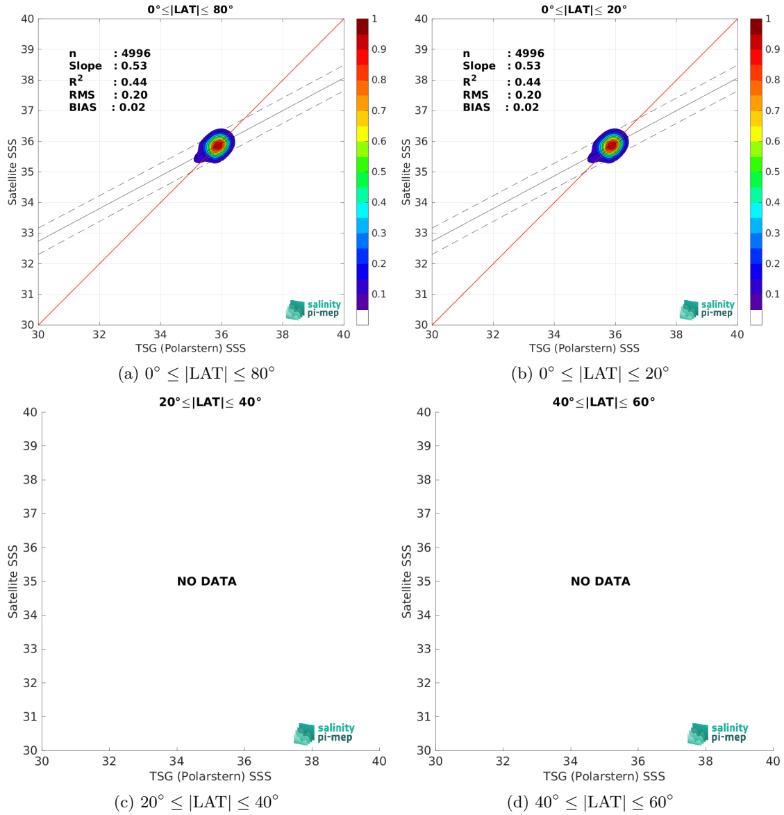
Figure 10: Contour maps of the concentration of SMOS SSS L4 v1 - Daily (CMEMS-CNR) SSS (y-axis) versus TSG (Polarstern) SSS (x-axis) at match-up pairs for different latitude bands. For each plot, the red line shows x=y . The black thin and dashed lines indicate a linear fit through the data cloud and the \pm 95\% confidence levels, respectively. The number match-up pairs n , the slope and R^2 coefficient of the linear fit, the root mean square (RMS) and the mean bias between satellite and in situ data are indicated for each latitude band in each plots.
