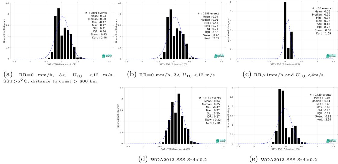
Figure 15: Normalized histogram of \Delta\text{SSS} (SMOS SSS L4 v1 - Daily (CMEMS-CNR) - TSG (Polarstern)) for 5 different subdatasets corresponding to: RR=0 mm/h, 3 < U_{10} < 12 m/s, SST>5°C, distance to coast > 800 km (a), RR=0 mm/h, 3 < U_{10} < 12 m/s (b), RR>1mm/h and U_{10} < 4 m/s (c), WOA2013 SSS Std<0.2 (d), WOA2013 SSS Std>0.2 (e).
