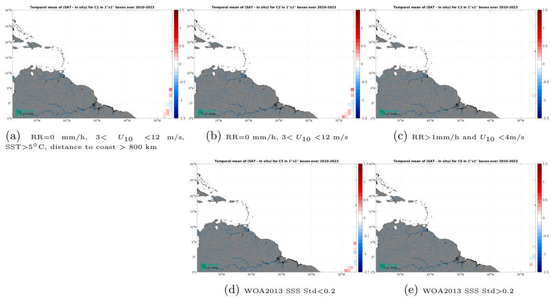
Figure 14: Temporal mean gridded over spatial boxes of size 1^\circ \times 1^\circ of \Delta SSS (SMOS SSS L4 v1 - Daily (CMEMS-CNR) - TSG (Polarstern)) for 5 different subdatasets corresponding to:RR=0 mm/h, 3 < U_{10} < 12 m/s, SST >5^\circ\text{C} , distance to coast > 800 km (a), RR=0 mm/h, 3 < U_{10} < 12 m/s (b), RR >1 mm/h and U_{10} < 4 m/s (c), WOA2013 SSS Std <0.2 (d), WOA2013 SSS Std >0.2 (e).
