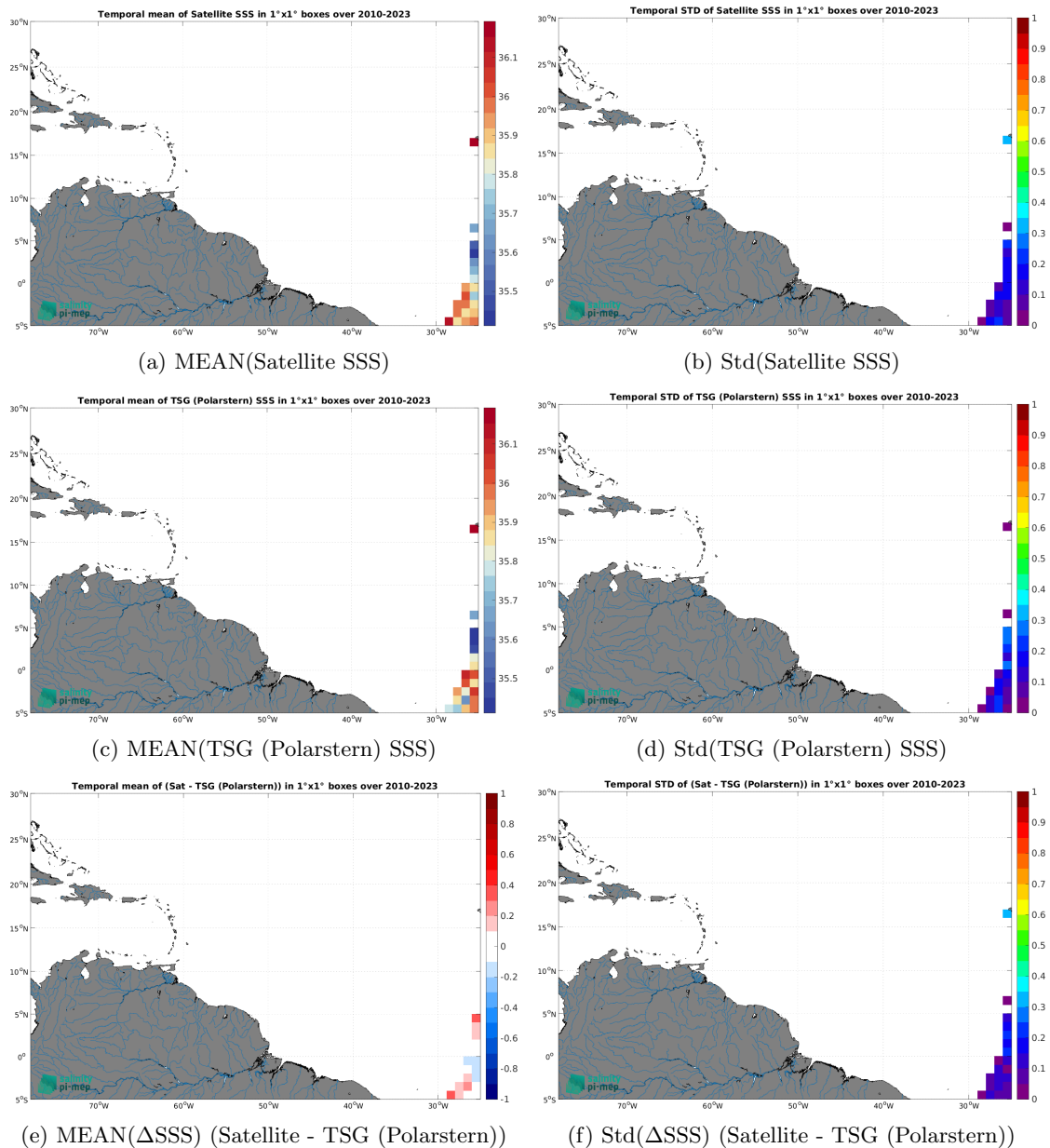
Figure 7: Temporal mean (left) and Std (right) of SSS from SMOS SSS L4 v1 - Daily (CMEMS-CNR) (top), TSG (Polarstern) (middle), and of \Delta SSS (Satellite - TSG (Polarstern)). Only match-up pairs are used to generate these maps.
