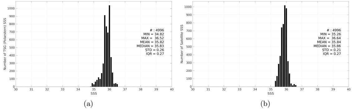
Figure 3: Histograms of SSS from TSG (Polarstern) (a) and SMOS SSS L4 v1 - Daily (CMEMS-CNR) (b) considering all match-up pairs per bins of 0.1 over the Amazon and Orinoco river plumes Pi-MEP region and for the full satellite product period.
