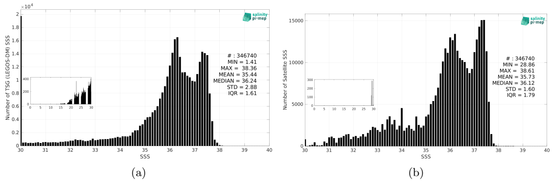
Figure 3: Histograms of SSS from TSG (LEGOS-DM) (a) and SMOS SSS L4 v1 - Daily (CMEMS-CNR) (b) considering all match-up pairs per bins of 0.1 over the Amazon and Orinoco river plumes Pi-MEP region and for the full satellite product period.
