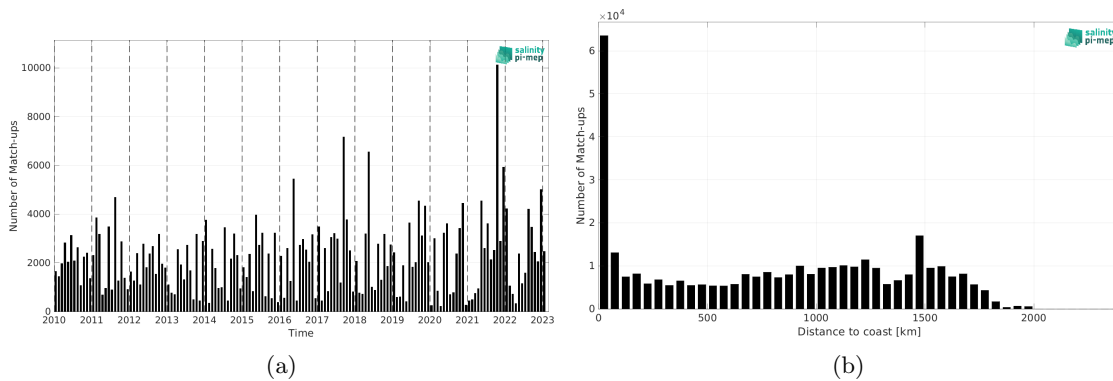
Figure 2: Number of match-ups between TSG (LEGOS-DM) and SMOS SSS L4 v1 - Daily (CMEMS-CNR) SSS as a function of time (a) and as function of the distance to coast (b) over the Amazon and Orinoco river plumes Pi-MEP region and for the full satellite product period.
