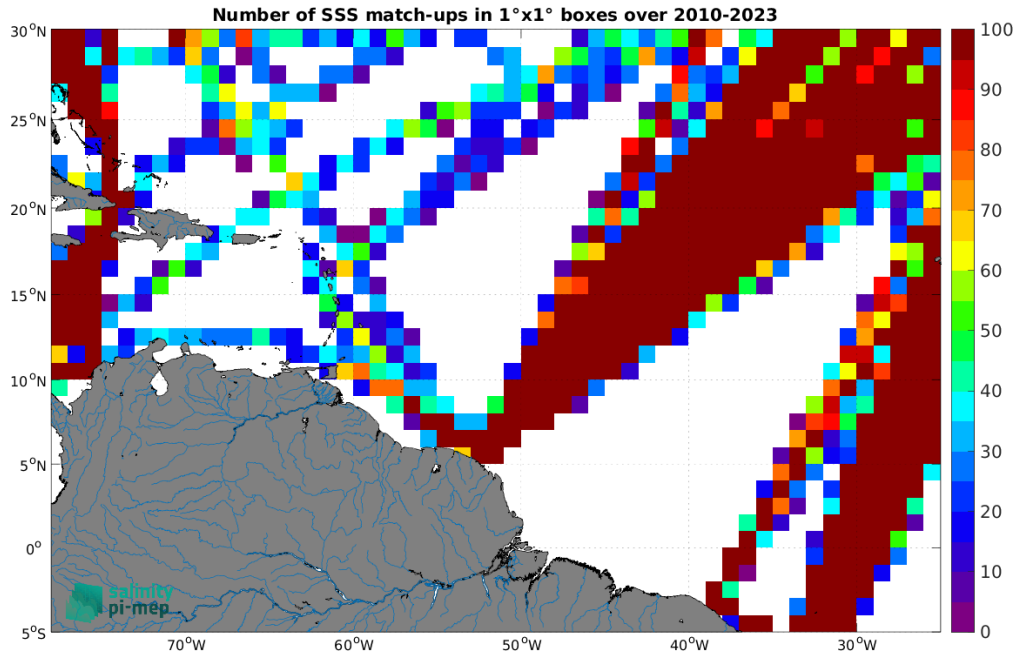
Figure 5: Number of SSS match-ups between TSG (LEGOS-DM) SSS and the SMOS SSS L4 v1 - Daily (CMEMS-CNR) SSS product for the Amazon and Orinoco river plumes Pi-MEP region over 1^\circ \times 1^\circ boxes and for the full satellite product period.
