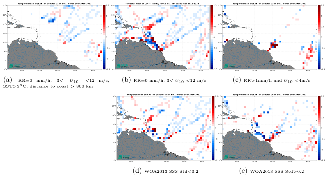
Figure 14: Temporal mean gridded over spatial boxes of size 1^\circ \times 1^\circ of \Delta\text{SSS} (SMOS SSS L4 v1 - Daily (CMEMS-CNR) - TSG (LEGOS-DM)) for 5 different subdatasets corresponding to:RR=0 mm/h, 3 < U_{10} < 12 m/s, SST >5^\circ\text{C} , distance to coast > 800 km (a), RR=0 mm/h, 3 < U_{10} < 12 m/s (b), RR >1 mm/h and U_{10} < 4 m/s (c), WOA2013 SSS Std <0.2 (d), WOA2013 SSS Std >0.2 (e).
