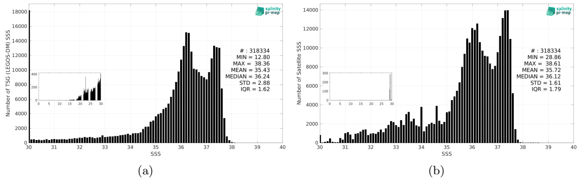
Figure 3: Histograms of SSS from TSG (LEGOS-DM) (a) and SMOS SSS L4 v1 - Daily (CMEMS-CNR) (b) considering all match-up pairs per bins of 0.1 over the Amazon and Orinoco river plumes Pi-MEP region and for the full satellite product period.
