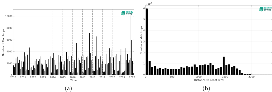
Figure 2: Number of match-ups between TSG (LEGOS-DM) and SMOS SSS L4 v1 - Daily (CMEMS-CNR) SSS as a function of time (a) and as function of the distance to coast (b) over the Amazon and Orinoco river plumes Pi-MEP region and for the full satellite product period.
