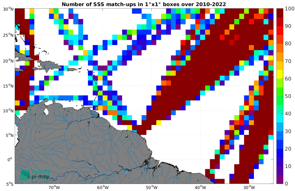
Figure 5: Number of SSS match-ups between TSG (LEGOS-DM) SSS and the SMOS SSS L4 v1 - Daily (CMEMS-CNR) SSS product for the Amazon and Orinoco river plumes Pi-MEP region over 1^{\circ} \times 1^{\circ} boxes and for the full satellite product period.
